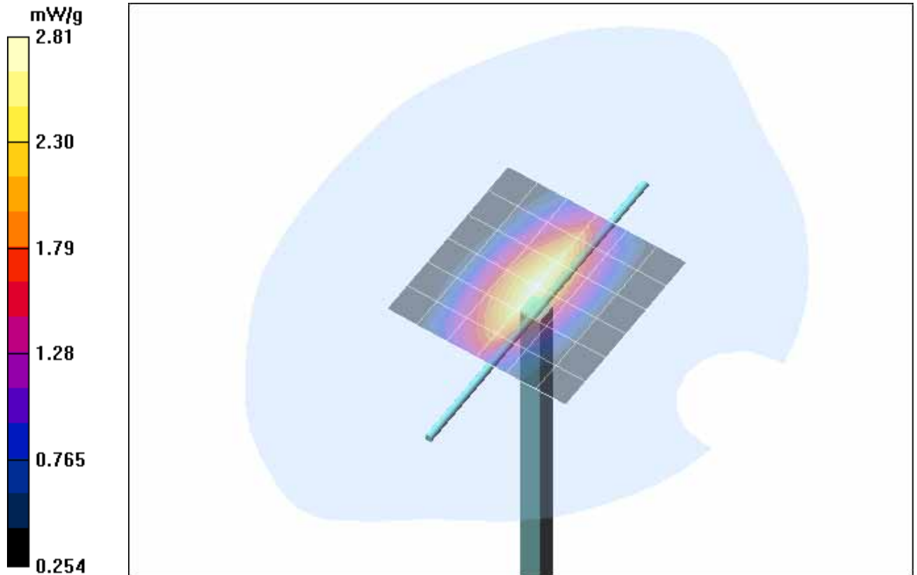
Fig. 12: Validation measurement 835MHz Body (GSM 850 and WCDMA V, January 16, 2006), coarse grid. Ambient Temperature: 21.2°C, Liquid Temperature: 20.1°C.
