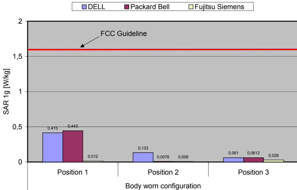
Fig. 9: The measured SAR values for the Option GT Max World in combination with the three host devices for GPRS 1900 at channel 661 in comparison to the FCC exposure limit.
