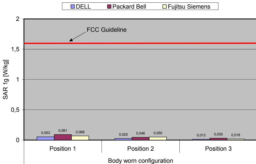
Fig. 11: The measured SAR values for the Option GT Max World in combination with the three host devices for ECDMA V (FDD) at channel 4183 in comparison to the FCC exposure limit.
