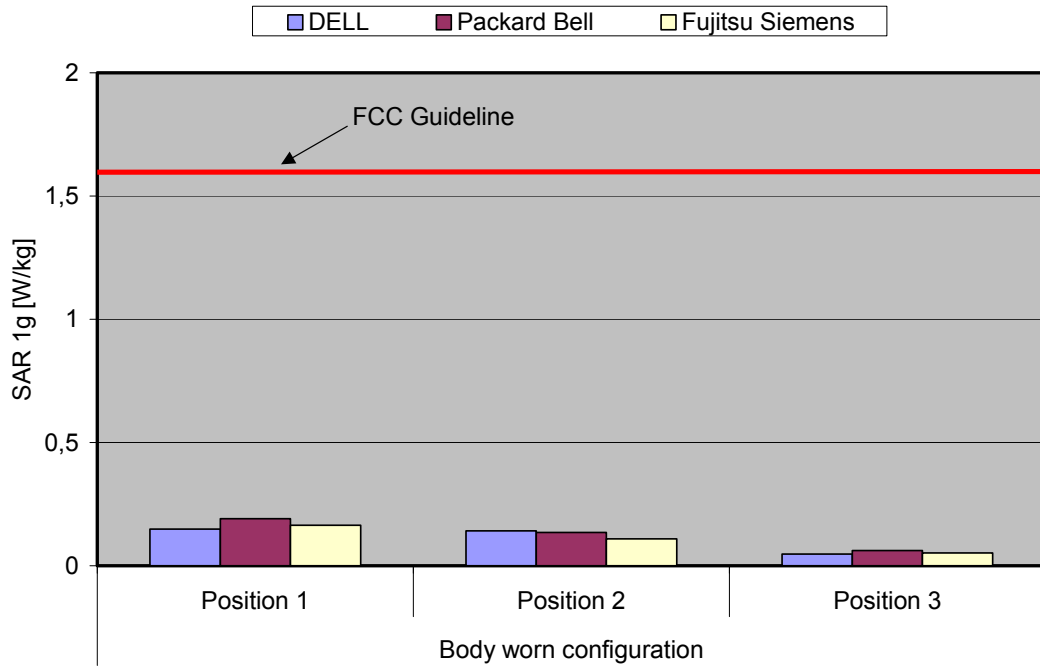
Fig. 8: The measured SAR values for the Option GT Max World in combination with the three host devices for GPRS 850 at channel 190 in comparison to the FCC exposure limit.
