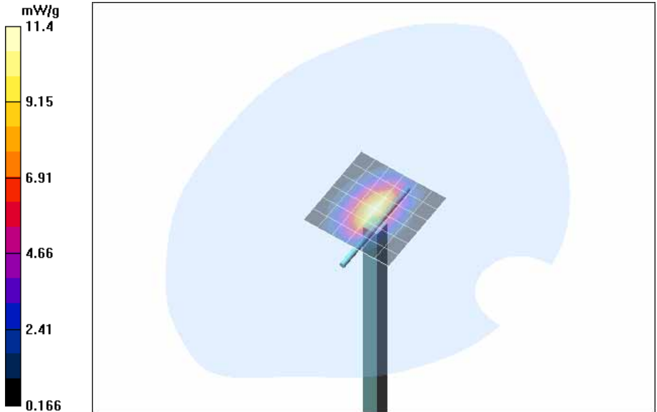
Fig. 13: Validation measurement 1900 MHz Body (PCS 1900 and WCDMA II January 12, 2006), coarse grid. Ambient Temperature: 21.2° C, Liquid Temperature: 20.4° C.
