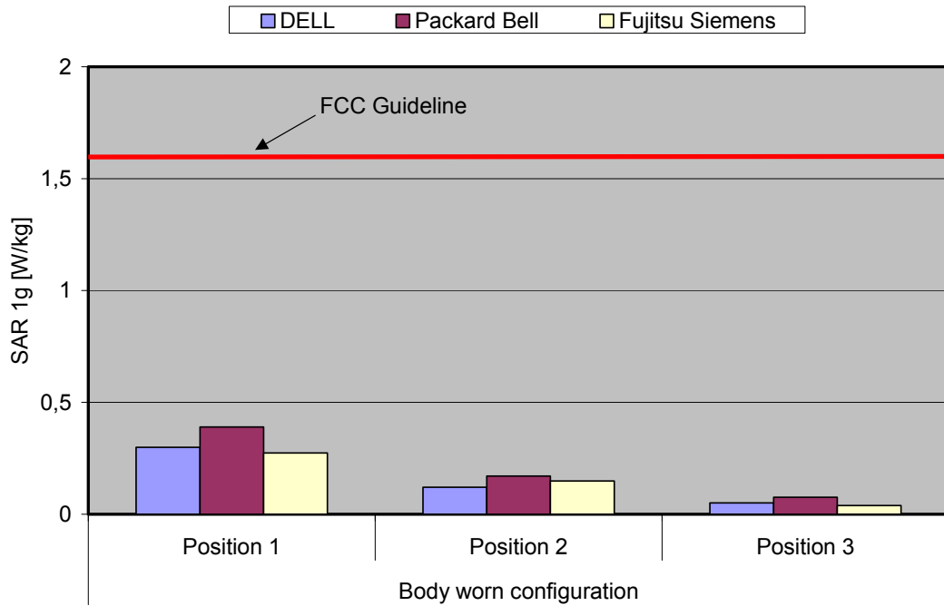
Fig. 10: The measured SAR values for the Option GT Max World in combination with the three host devices WCDMA II (FDD) at channel 187 in comparison to the FCC exposure limit.
