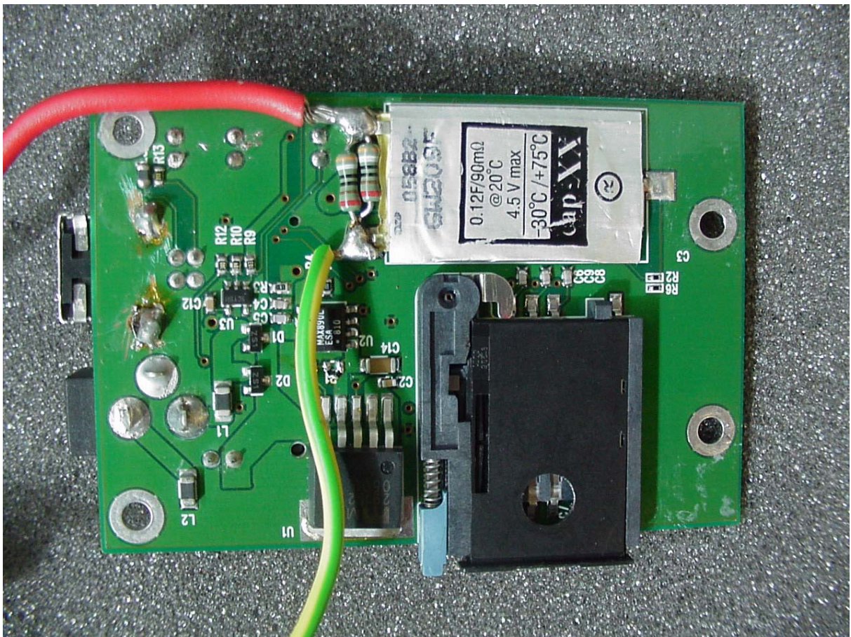
Photo 6: Cradle (rear side)
