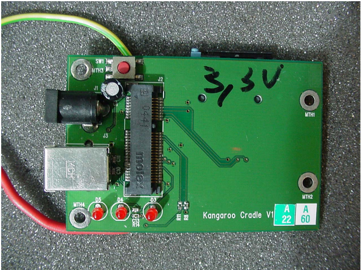
Photo 5: Cradle (front side)
