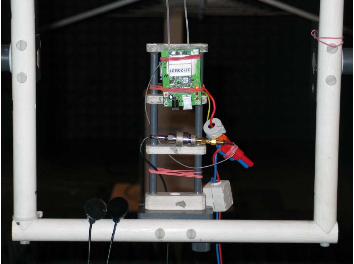
Photo 3: Setup for radiated tests (EUT operated in a cradle and with external antenna)
