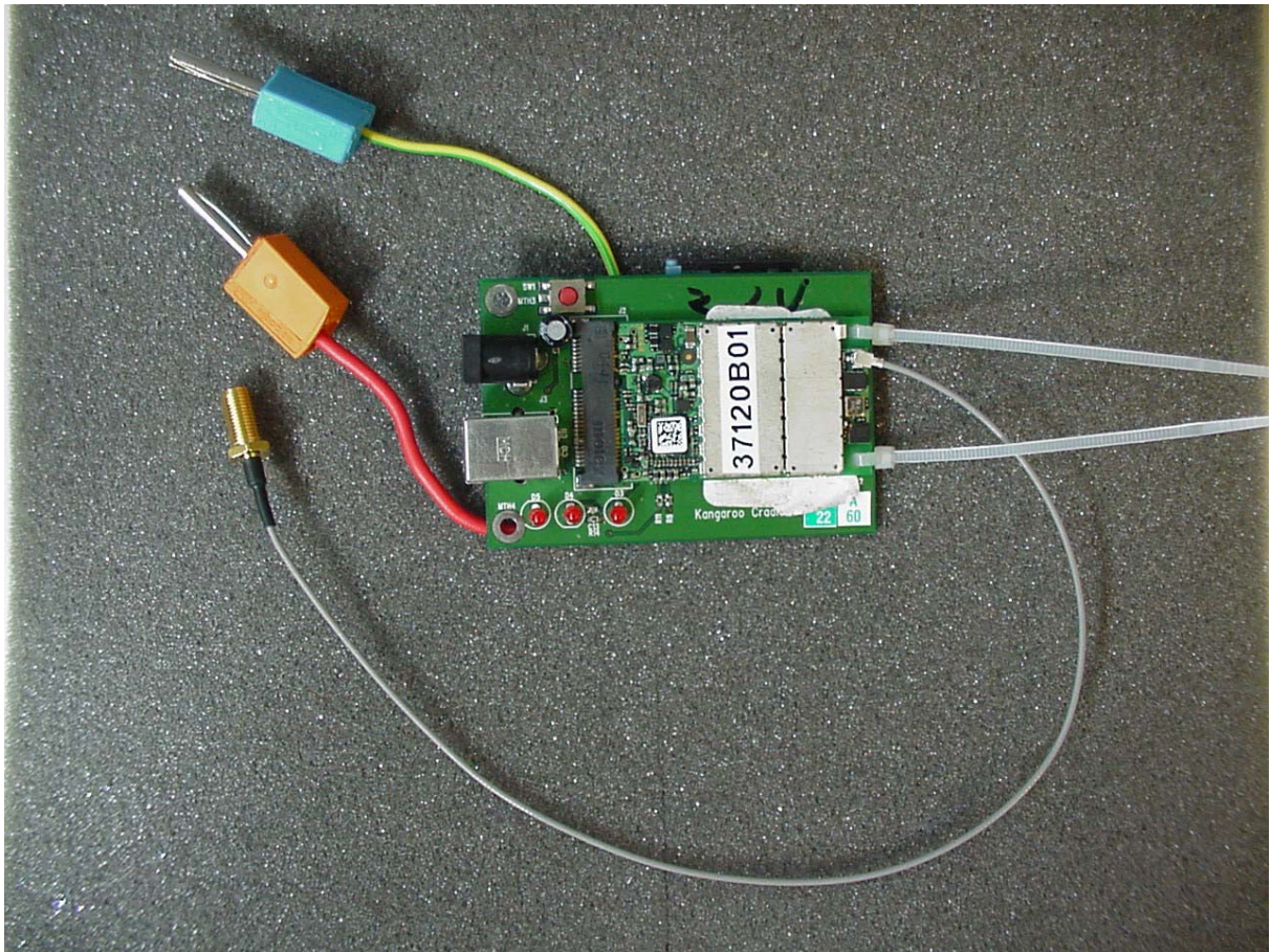
Photo 4: Setup for conducted tests (EUT operated in a cradle, with temporary antenna adapter to SMA)
