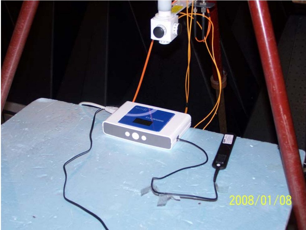
Photograph 5: Measurements in the anechoic chamber: Test Set-up
