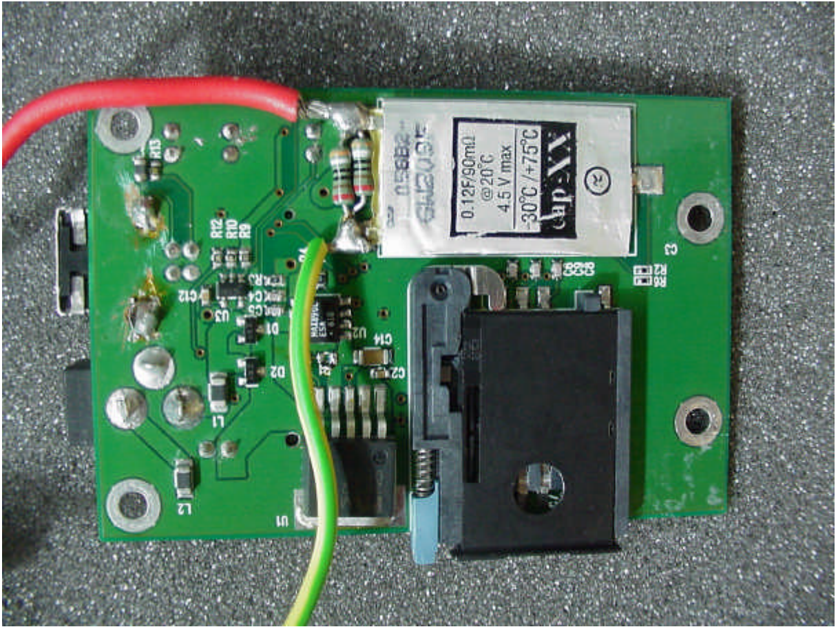
Photo 9: Cradle (rear side)
