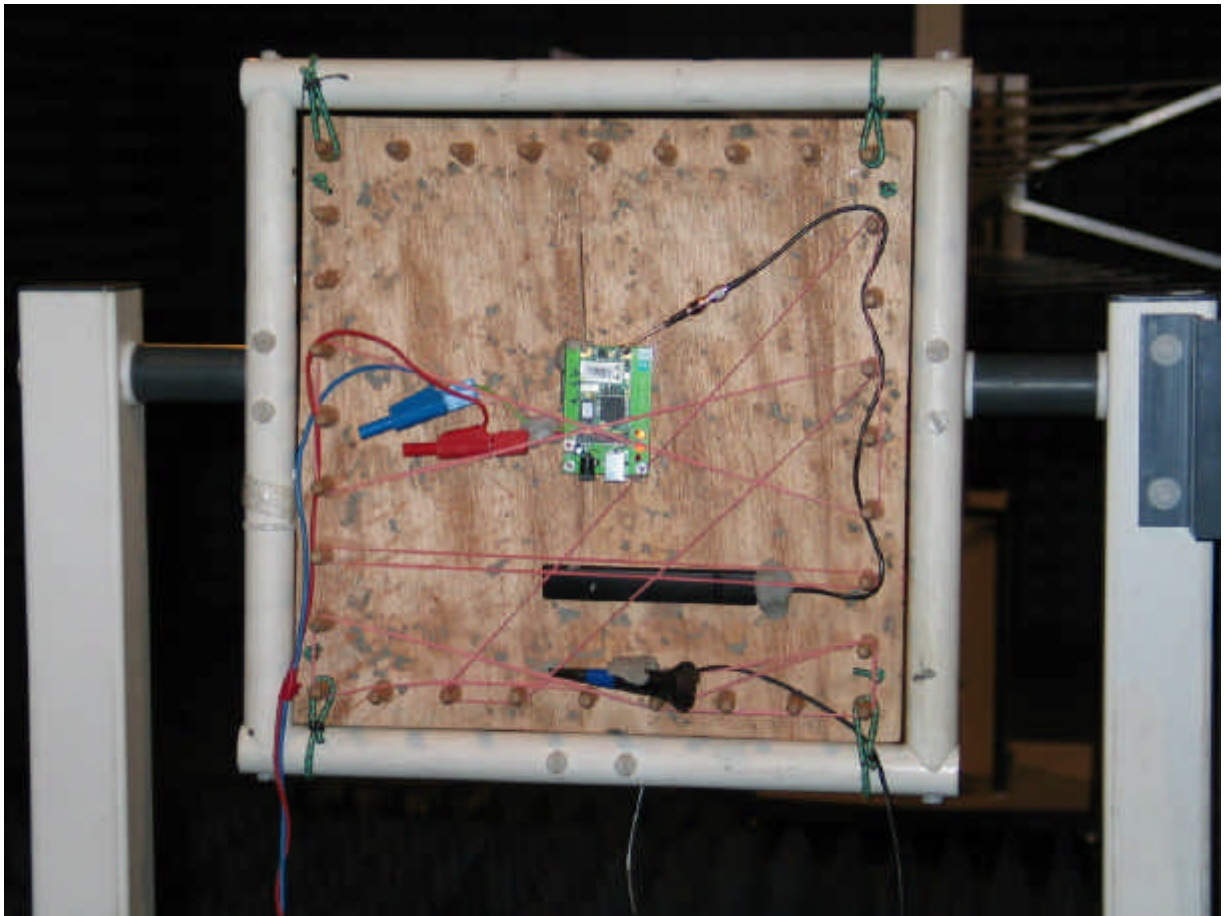
Photo 6: Setup for radiated tests (EUT A operated in a cradle and with external antenna)
