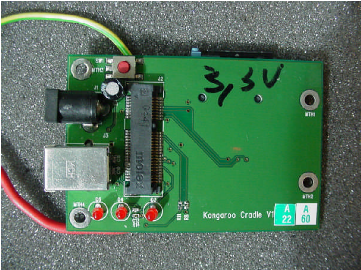
Photo 8: Cradle AE1 (front side)
