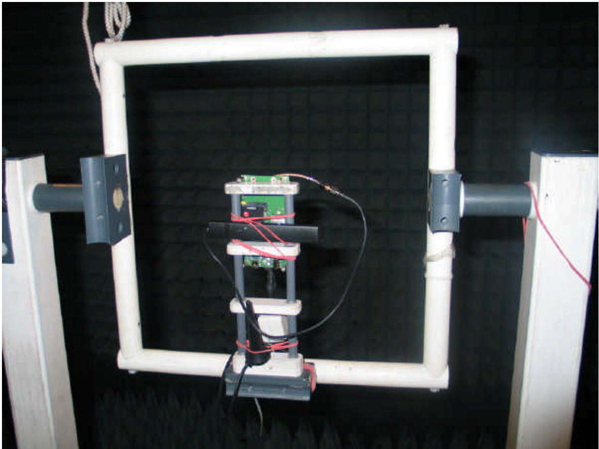
Photo 7: Setup for radiated tests (EUT C operated in a cradle and with external antenna)
