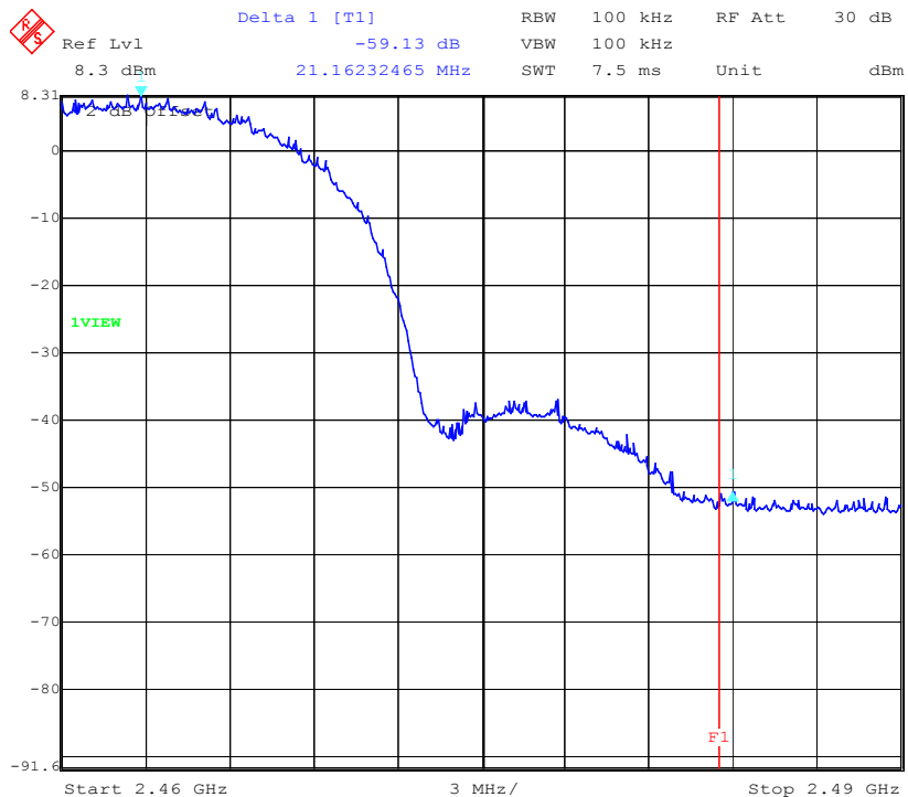
Plot 2, highest channel
