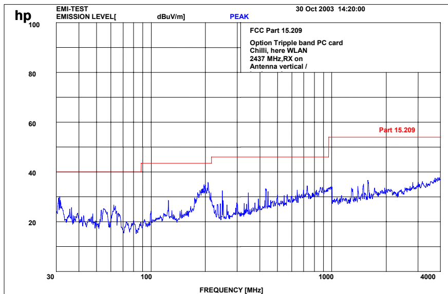
Plot 1: 0.03 - 4 GHz vertical / horizontal (receiver)
