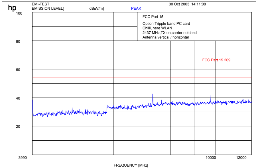
Plot 5: 4- 12 GHz (middle channel)
