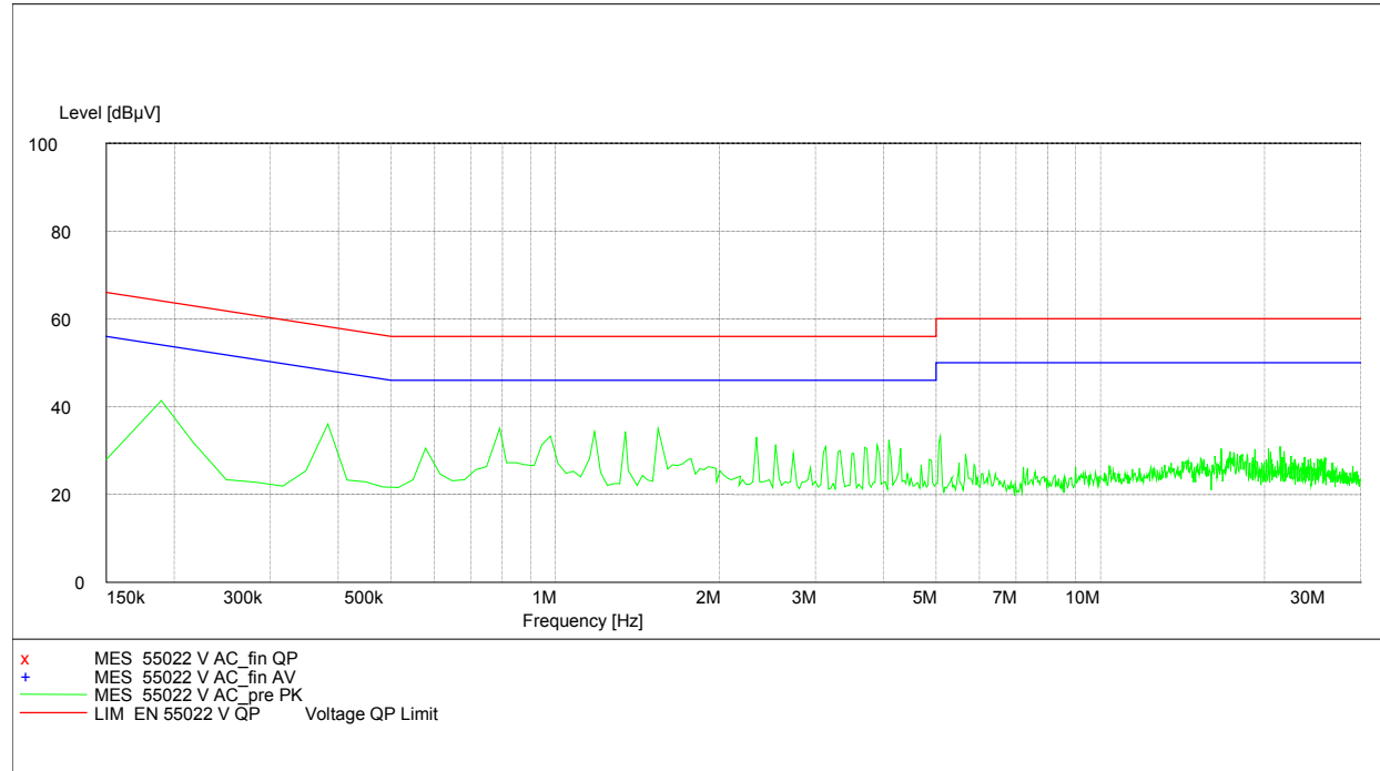
Plot 2 RX: CISPR 22
