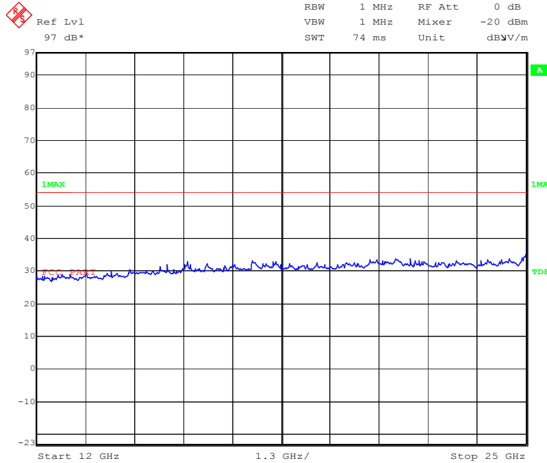
Plot 3: 12- 25 GHz (receiver)
