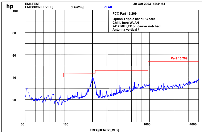
Plot 1: 0.03 - 4 GHz vertical / horizontal (lowest channel)
