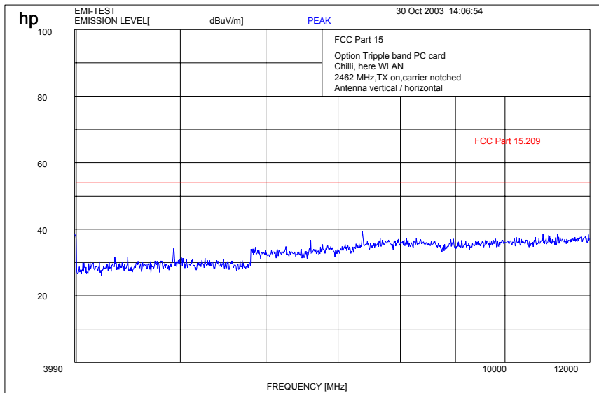
Plot 7: 4- 12 GHz (highest channel)
