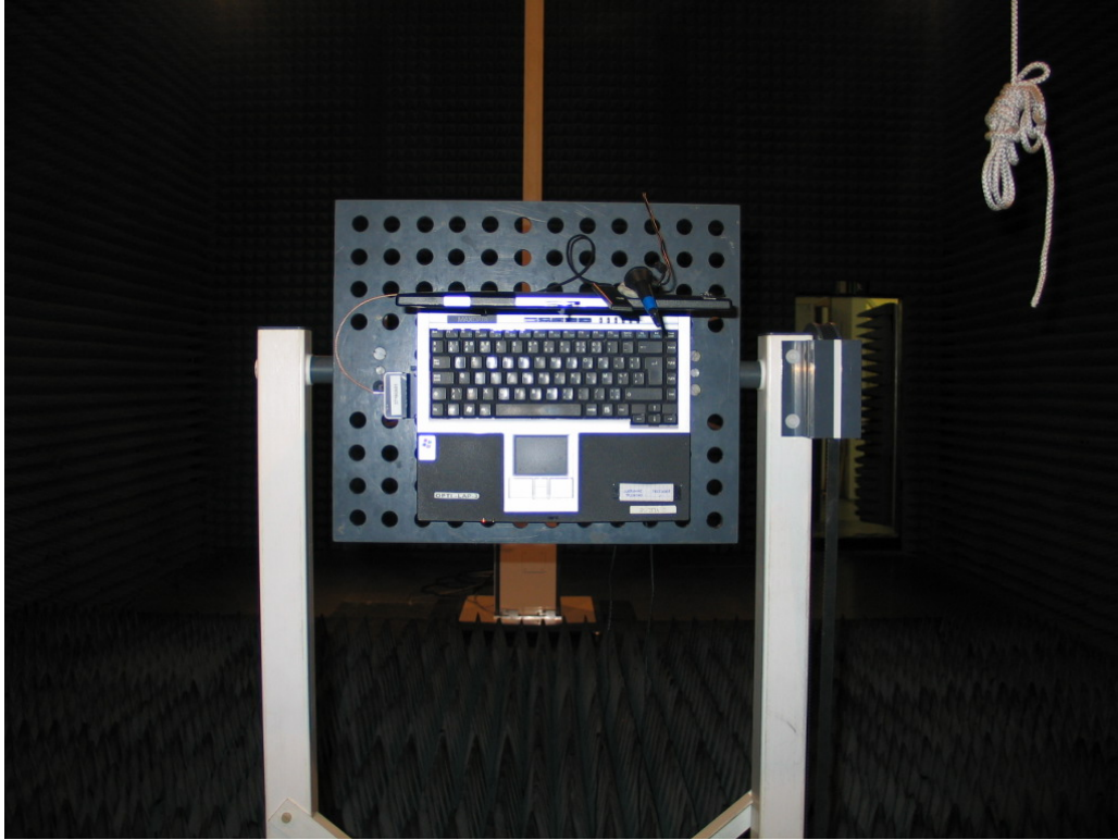
Photo 1: Setup in the anechoic chamber
