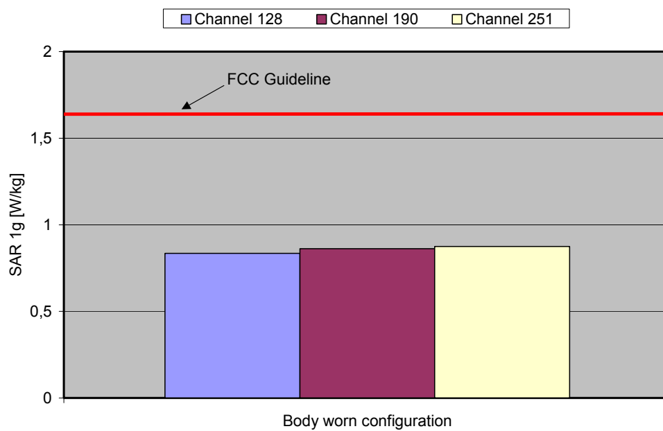
Fig. 10: The measured SAR values for the Option GT0201 in combination with the Toshiba SA50-110 Notebook for GPRS 850 in comparison to the FCC exposure limit..
