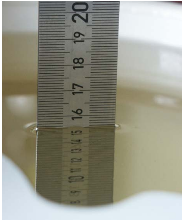
Fig. 30: Liquid depth for GPRS 850 and WCDMA V Body measurements.
