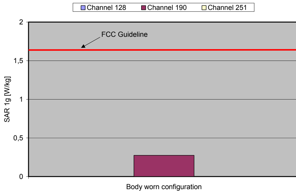
Fig. 8: The measured SAR values for the Option GT0201 in combination with the DELL Latitude C810 Notebook for GPRS 850 in comparison to the FCC exposure limit.
