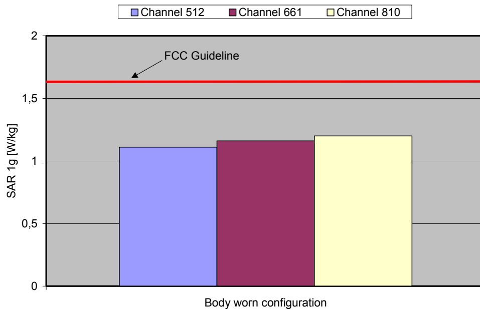
Fig. 12: The measured SAR values for the Option GT0201 in combination with the Packard Bell Easy Note Notebook for GPRS 1900 in comparison to the FCC exposure limit.
