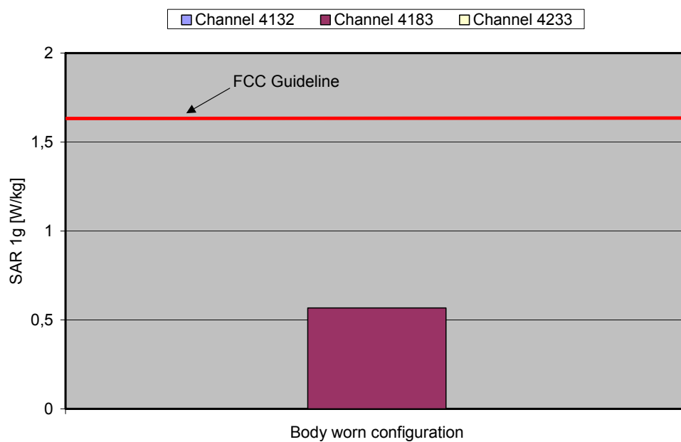
Fig. 19: The measured SAR values for the Option GT0201 in combination with the Toshiba SA50-110 Notebook for WCDMA V (FDD) in comparison to the FCC exposure limit..
