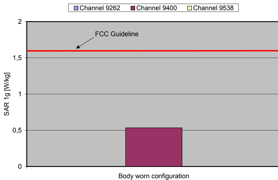
Fig. 15: The measured SAR values for the Option GT0201 in combination with the Packard Bell Easy Note Notebook for WCDMA II (FDD) in comparison to the FCC exposure limit.
