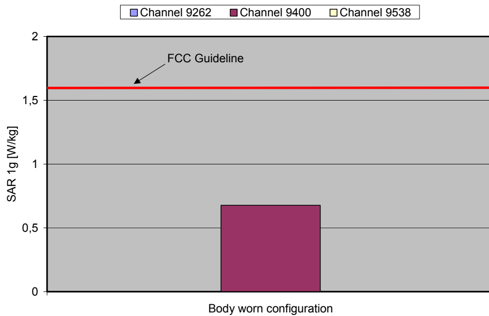
Fig. 14: The measured SAR values for the Option GT0201 in combination with the DELL Latitude C810 Notebook for WCDMA II (FDD) in comparison to the FCC exposure limit.
