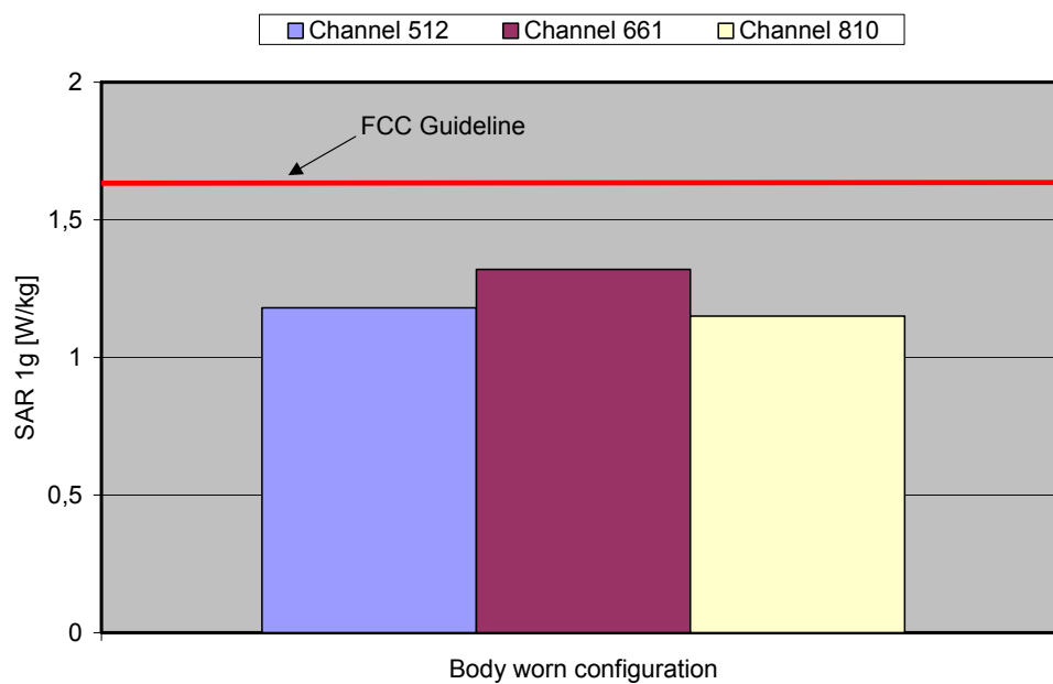
Fig. 11: The measured SAR values for the Option GT0201 in combination with the DELL Latitude C810 Notebook for GPRS 1900 in comparison to the FCC exposure limit.
