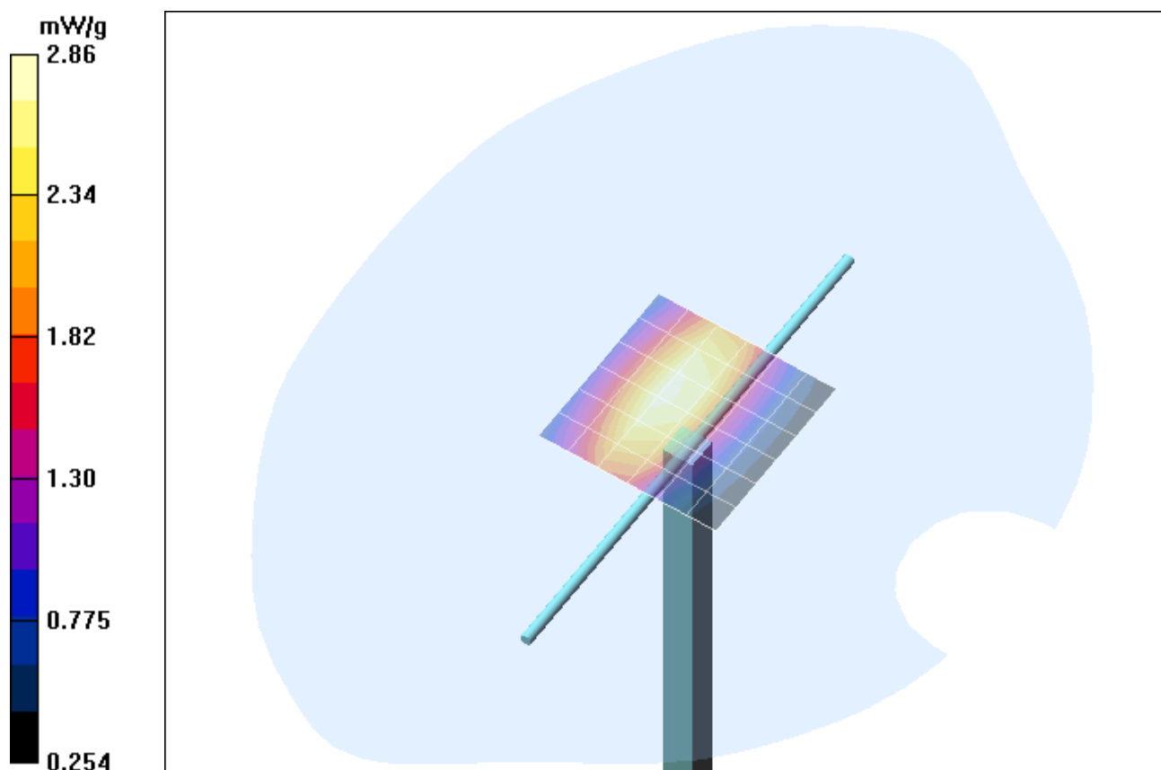
Fig. 20: Validation measurement 835 MHz Body (GSM 850 and WCDMA V, November 08, 2006), coarse grid. Ambient Temperature: 21.1°C, Liquid Temperature: 20.5°C.
