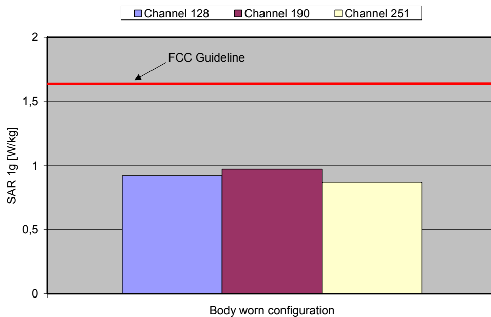
Fig. 9: The measured SAR values for the Option GT0201 in combination with the Packard Bell Easy Note Notebook for GPRS 850 in comparison to the FCC exposure limit.
