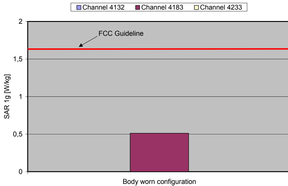
Fig. 18: The measured SAR values for the Option GT0201 in combination with the Packard Bell Easy Note Notebook for WCDMA V (FDD) in comparison to the FCC exposure limit.
