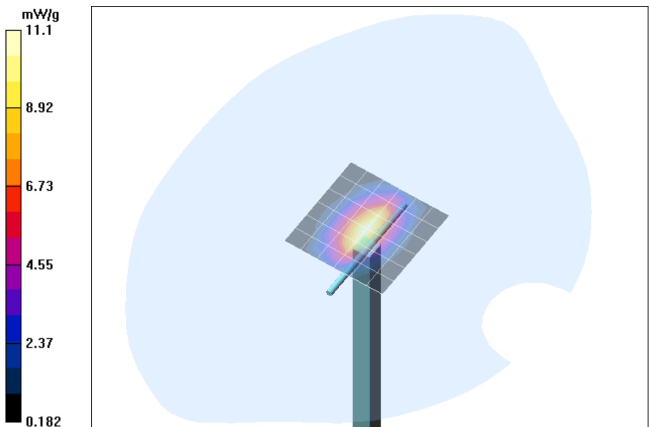
Fig. 21: Validation measurement 1900 MHz Body (GSM 1900 and WCDMA II, November 09, 2006), coarse grid. Ambient Temperature: 21.2°C, Liquid Temperature: 20.5°C.
