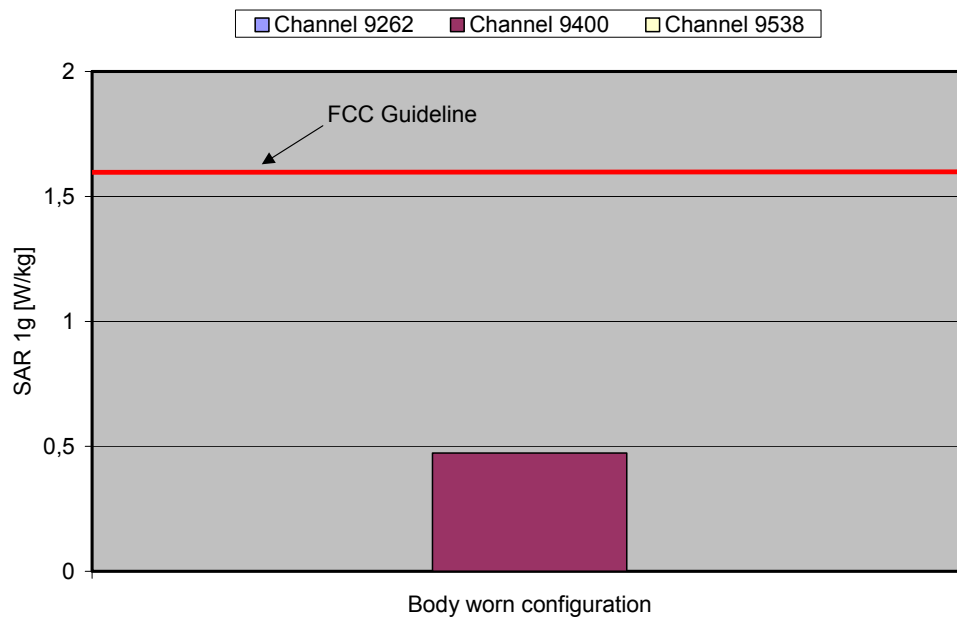
Fig. 16: The measured SAR values for the Option GT0201 in combination with the Toshiba SA50-110 Notebook for WCDMA II (FDD) in comparison to the FCC exposure limit..
