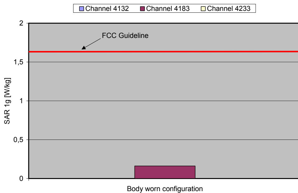
Fig. 17: The measured SAR values for the Option GT0201 in combination with the DELL Latitude C810 Notebook for WCDMA V (FDD) in comparison to the FCC exposure limit.
