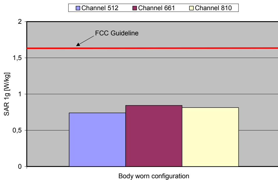
Fig. 13: The measured SAR values for the Option GT0201 in combination with the Toshiba SA50-110 Notebook for GPRS 1900 in comparison to the FCC exposure limit..
