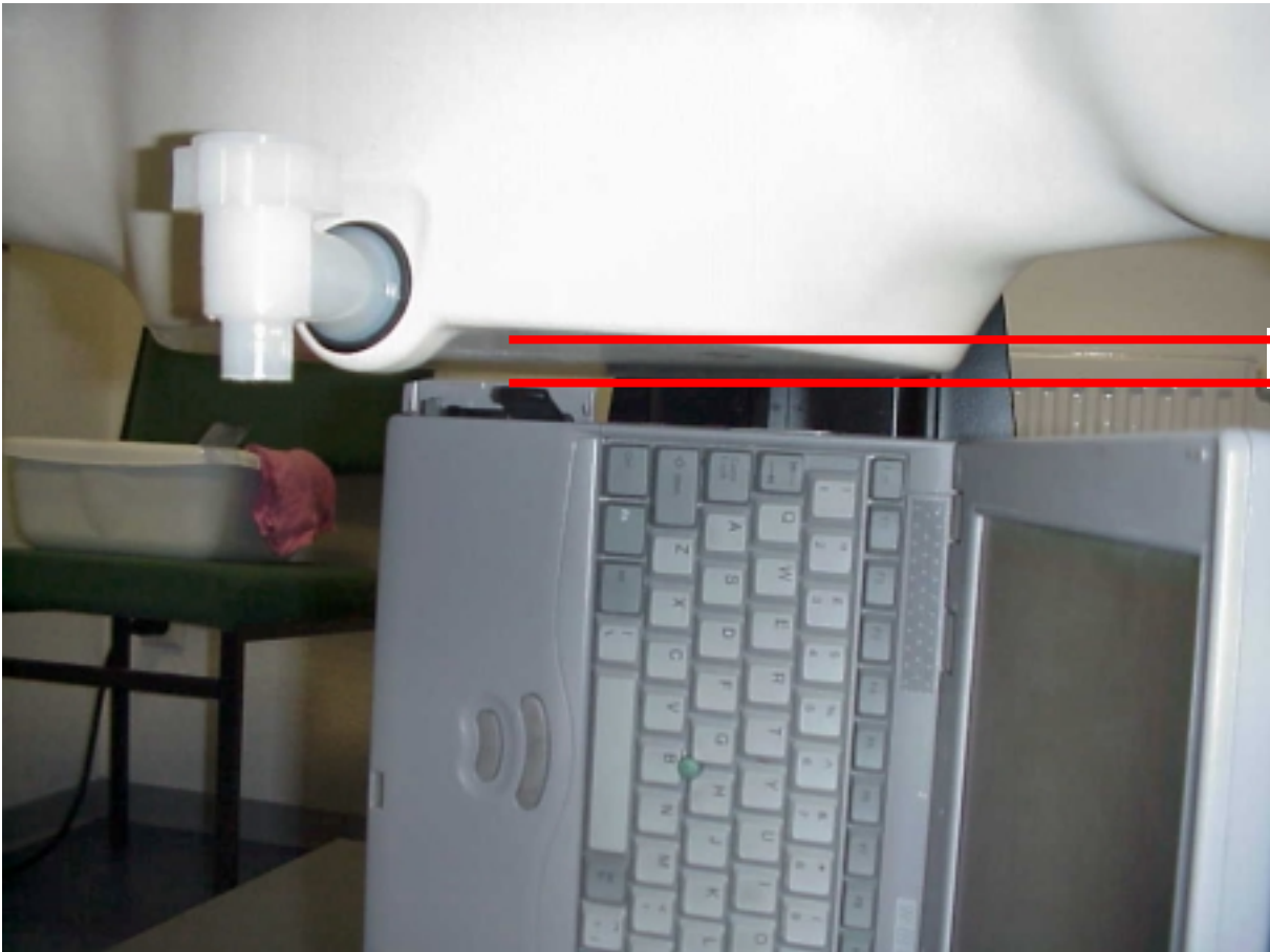
Photo 2: Position left side on the flat phantom (body SAR measurement)
