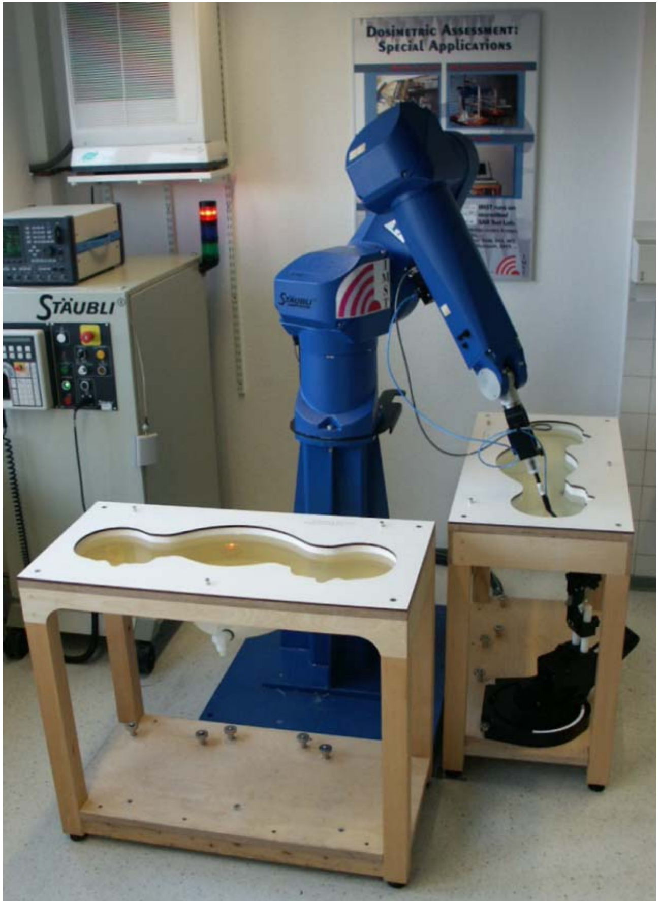
Fig. 5: The measurement set-up with two SAM phantoms containing tissue simulating liquid.
