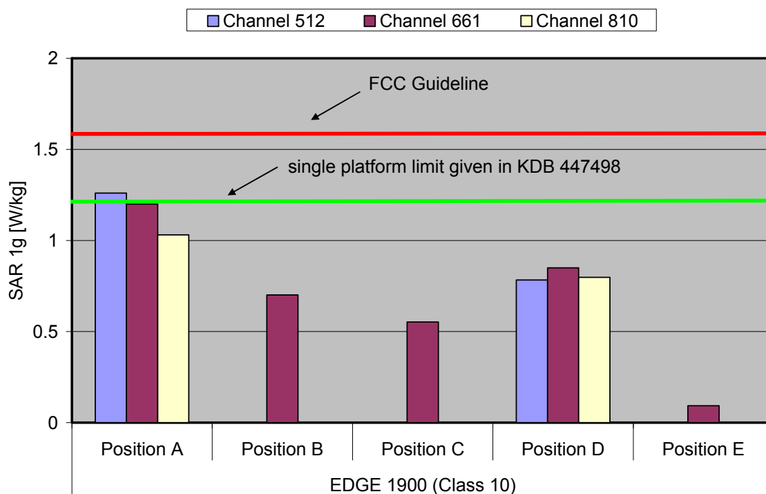
Fig. 9: The measured SAR values for the Option GI0461 for EDGE 1900 (Class 10) in comparison to the FCC exposure limit.
