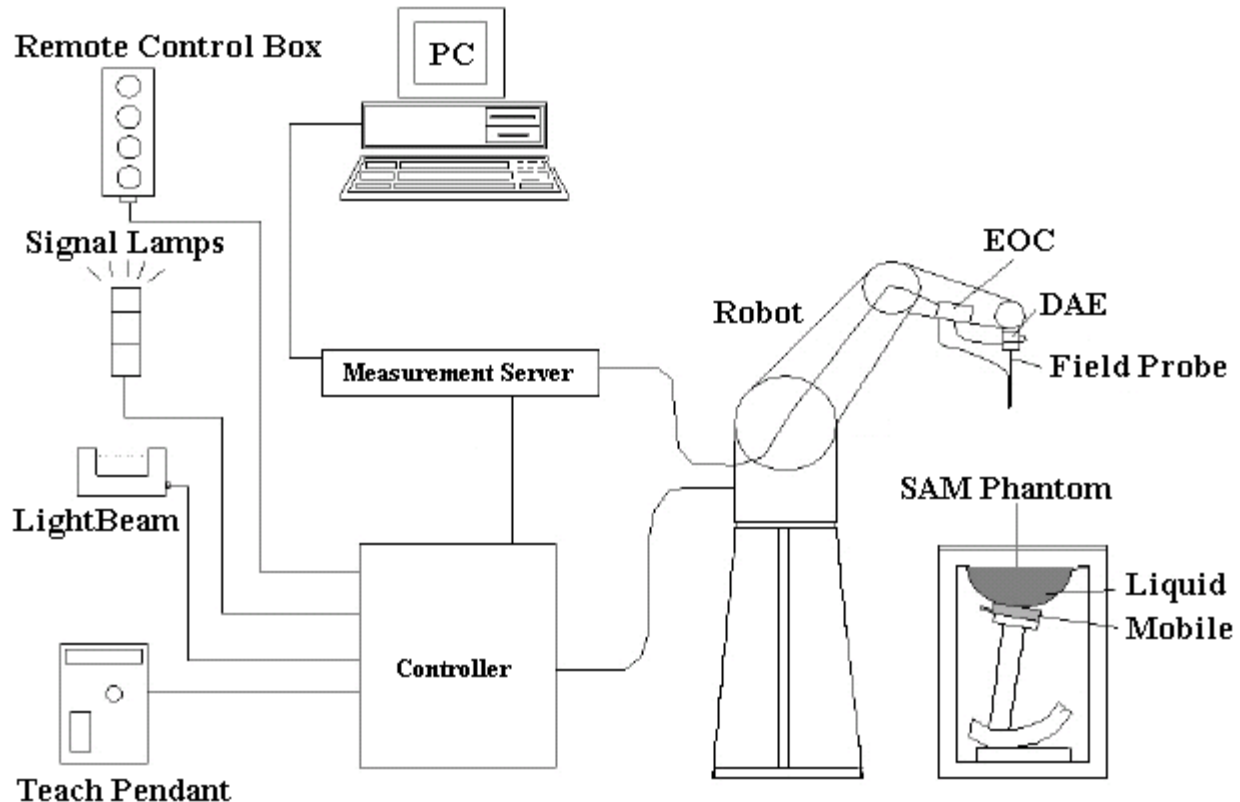
Fig. 4: The DASY4 measurement system.
