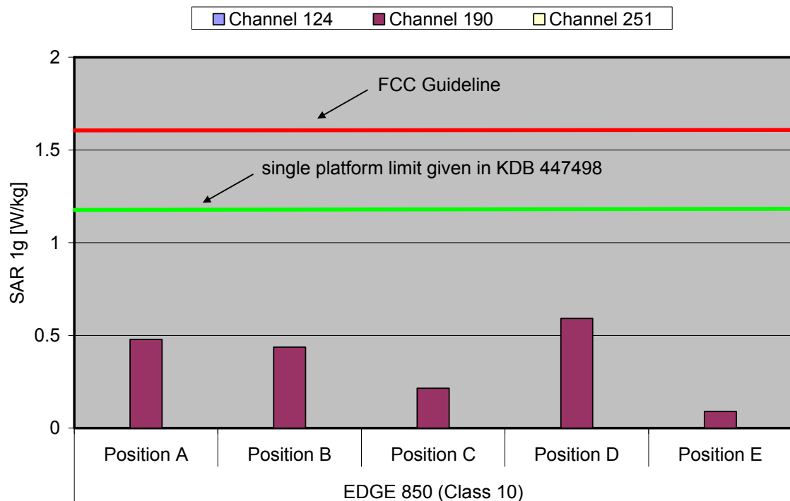
Fig. 7: The measured SAR values for the Option GI0461 for EDGE 850 (Class 10) in comparison to the FCC exposure limit.
