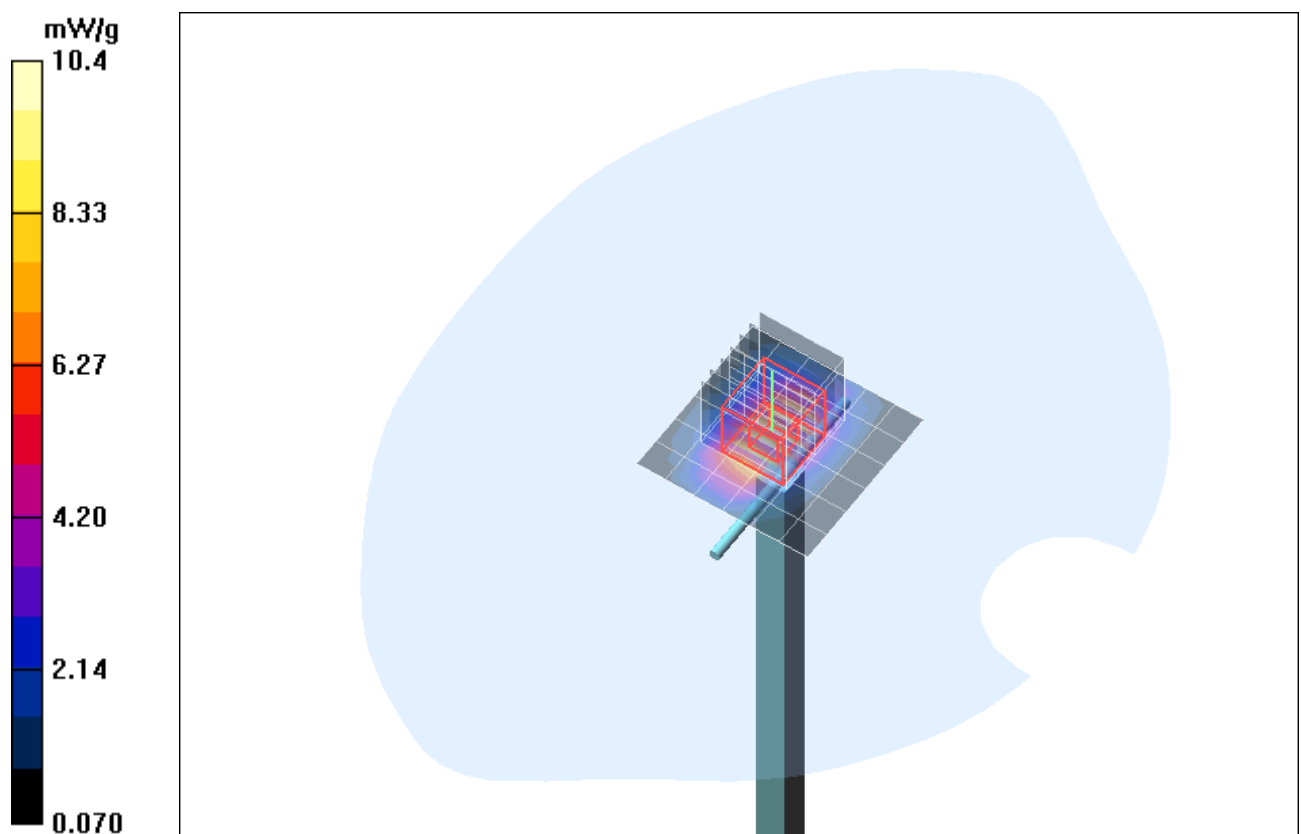
Fig. 15: Validation measurement 1900 MHz Body (WCDMA II, September 28, 2009), coarse grid. Ambient Temperature: 20.8°C, Liquid Temperature: 20.6°C.
