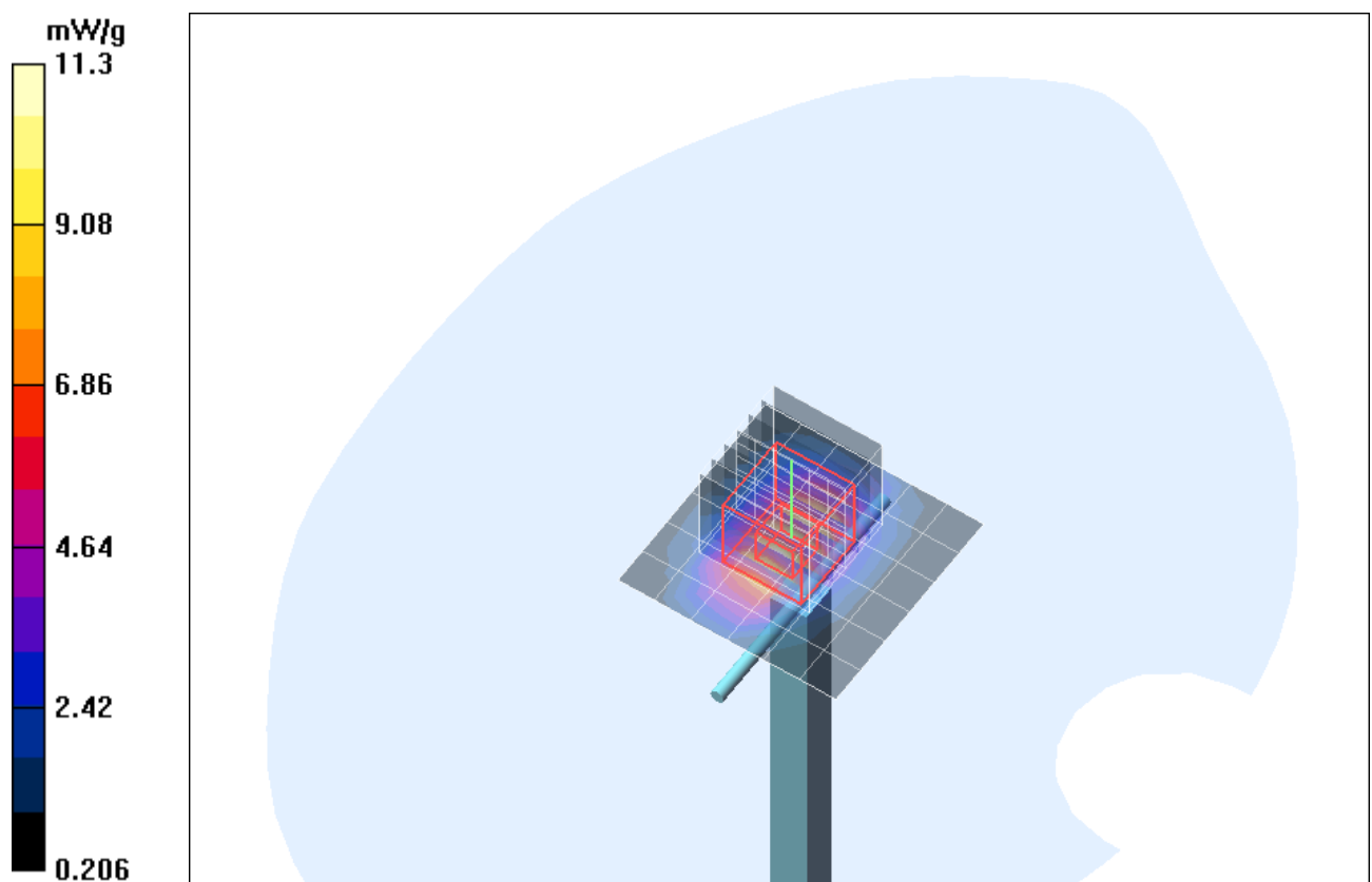
Fig. 14: Validation measurement 1900 MHz Body (GPRS/EDGE 1900, September 29, 2009), coarse grid. Ambient Temperature: 21.2°C, Liquid Temperature: 20.8°C.
