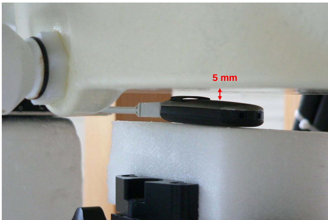
Fig. 21: Position B with the Fujitsu Siemens Amilo Pro.
