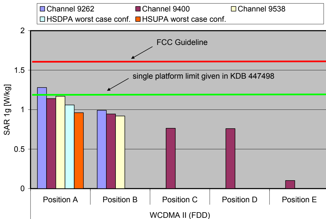
Fig. 11: The measured SAR values for the Option GI0461 for WCDMA II (FDD) in comparison to the FCC exposure limit.
