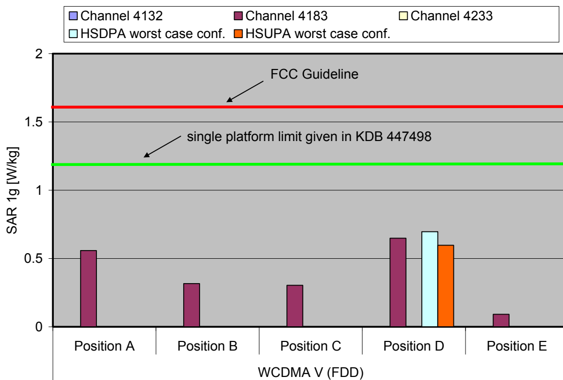
Fig. 10: The measured SAR values for the Option GI0461 for WCDMA V (FDD) in comparison to the FCC exposure limit.
