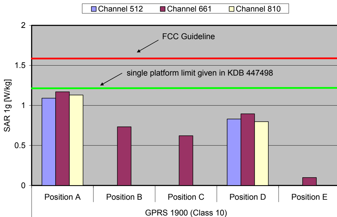
Fig. 8: The measured SAR values for the Option GI0461 for GPRS 1900 (Class 10) in comparison to the FCC exposure limit.
