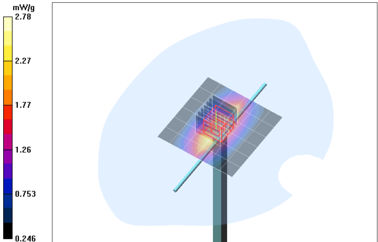
Fig. 12: Validation measurement 835 MHz Body (GPRS/EDGE 850, October 01, 2009), coarse grid. Ambient Temperature: 21.5°C, Liquid Temperature: 21.1°C.
