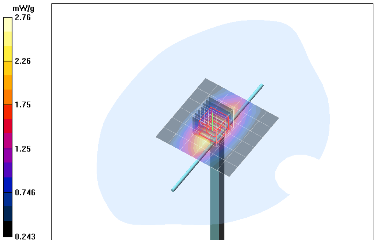
Fig. 13: Validation measurement 835 MHz Body (WCDMA V (FDD), September 30, 2009), coarse grid. Ambient Temperature: 21.2°C, Liquid Temperature: 20.8°C.
