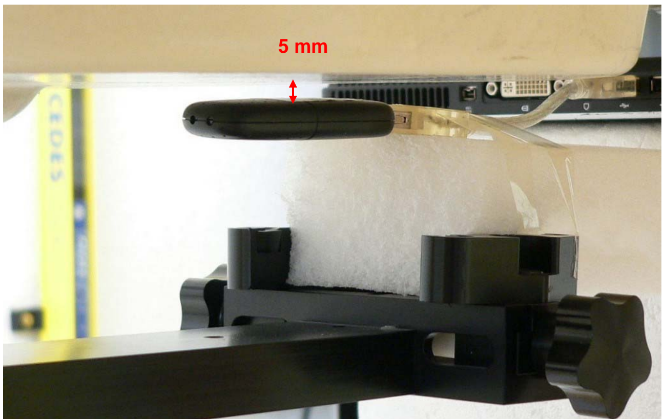
Fig. 17: Position B with the Fujitsu Siemens Amilo Pro.
