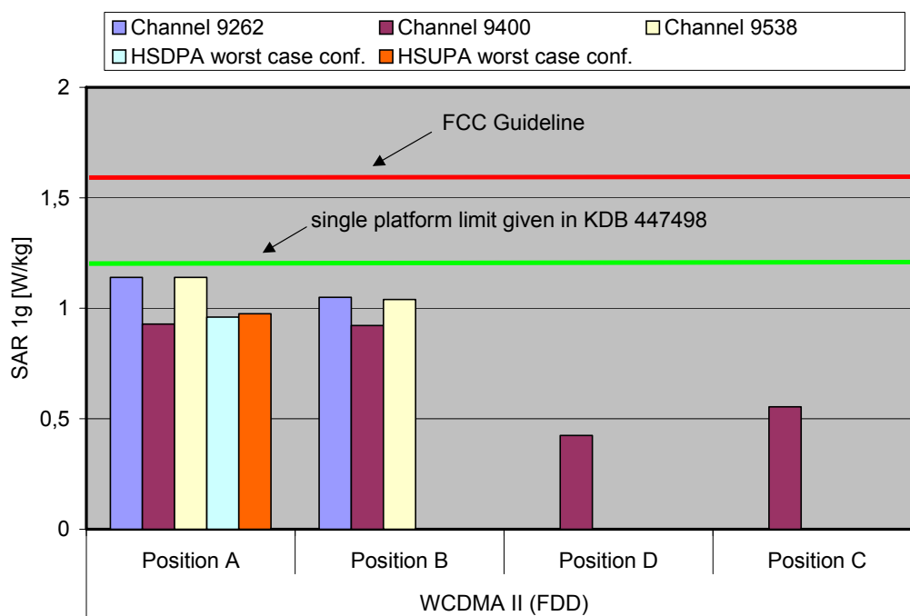
Fig. 8: The measured SAR values for the Option iCON451 for WCDMA II (FDD) in comparison to the FCC exposure limit.
