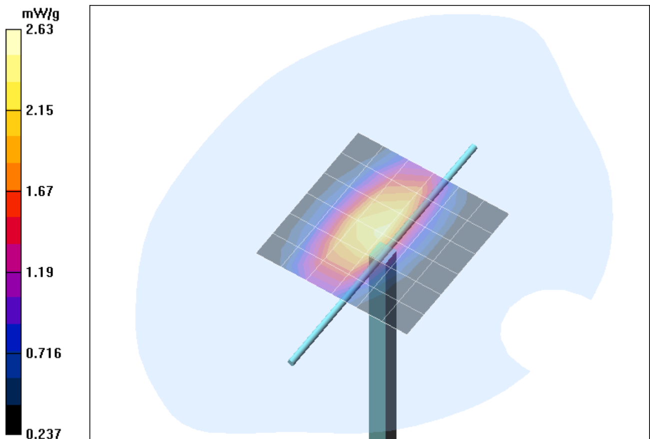
Fig. 9: Validation measurement 835 MHz Body (EDGE/GPRS 850 and WCDMA V, January 26, 2009), coarse grid. Ambient Temperature: 21.6°C, Liquid Temperature: 20.9°C.
