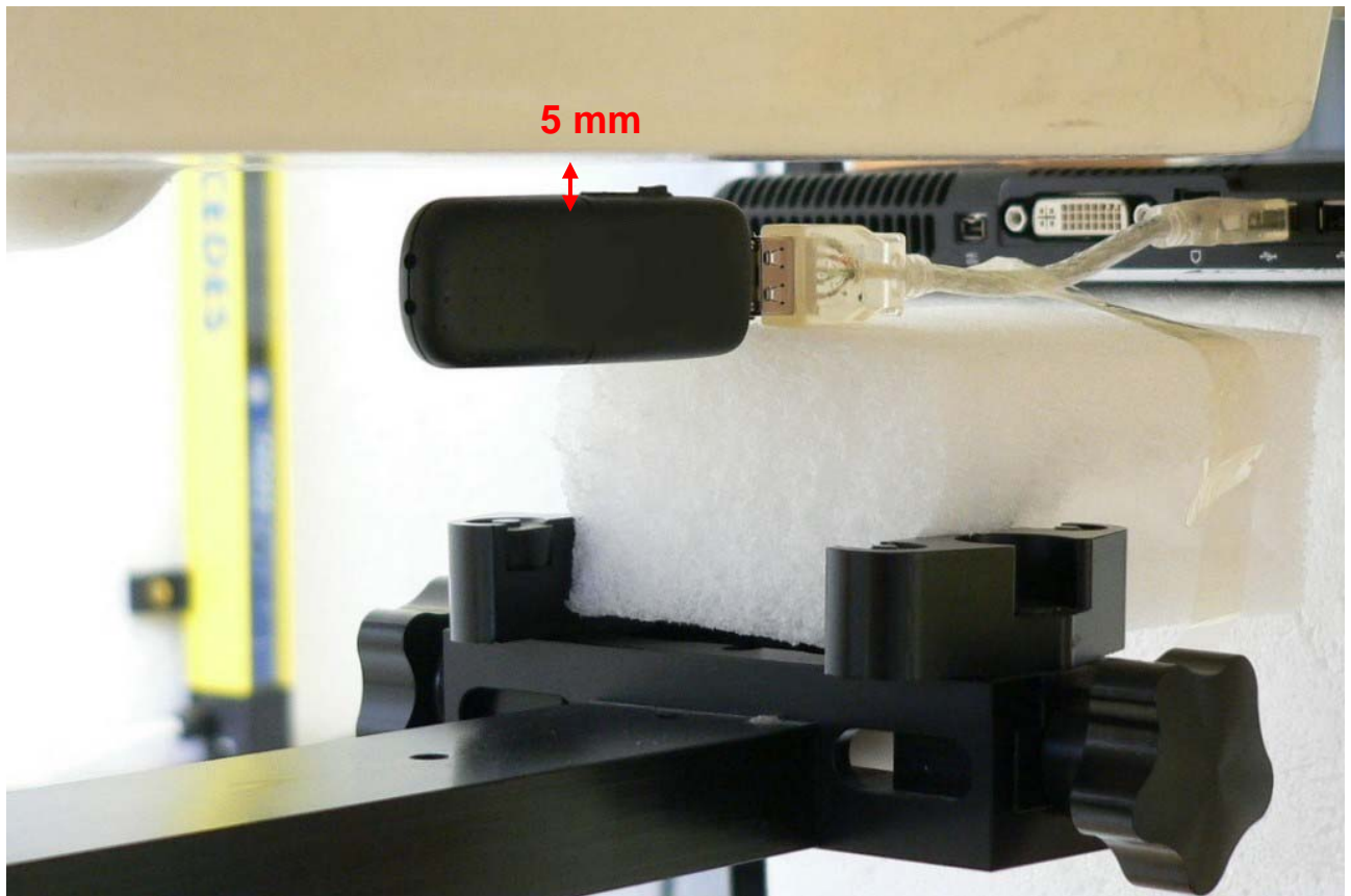
Fig. 18: Position D with the Fujitsu Siemens Amilo Pro.
