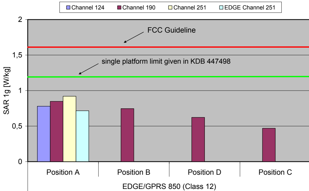
Fig. 5: The measured SAR values for the Option iCON451 for EDGE/GPRS 850 (Class 12) in comparison to the FCC exposure limit.
