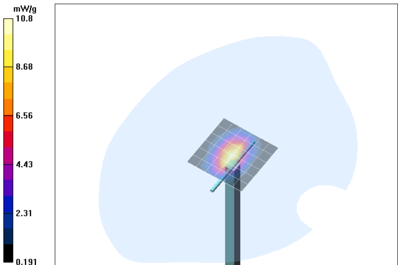
Fig. 10: Validation measurement 1900 MHz Body (EDGE/GPRS 1900, January 22, 2009), coarse grid. Ambient Temperature: 21.4°C, Liquid Temperature: 21.0°C.
