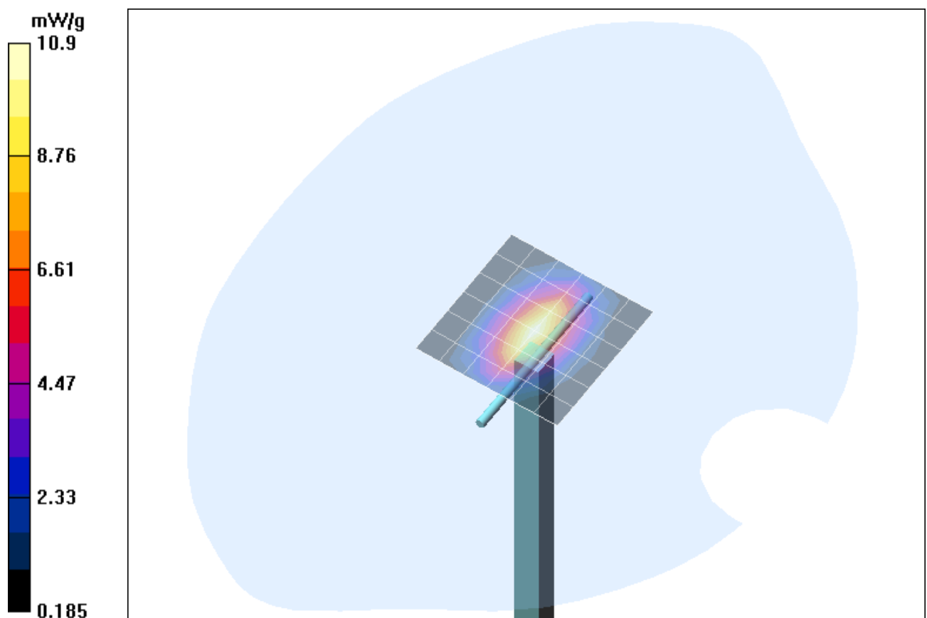
Fig. 11: Validation measurement 1900 MHz Body (WCDMA II, January 21, 2009), coarse grid. Ambient Temperature: 21.4°C, Liquid Temperature: 20.9°C.
