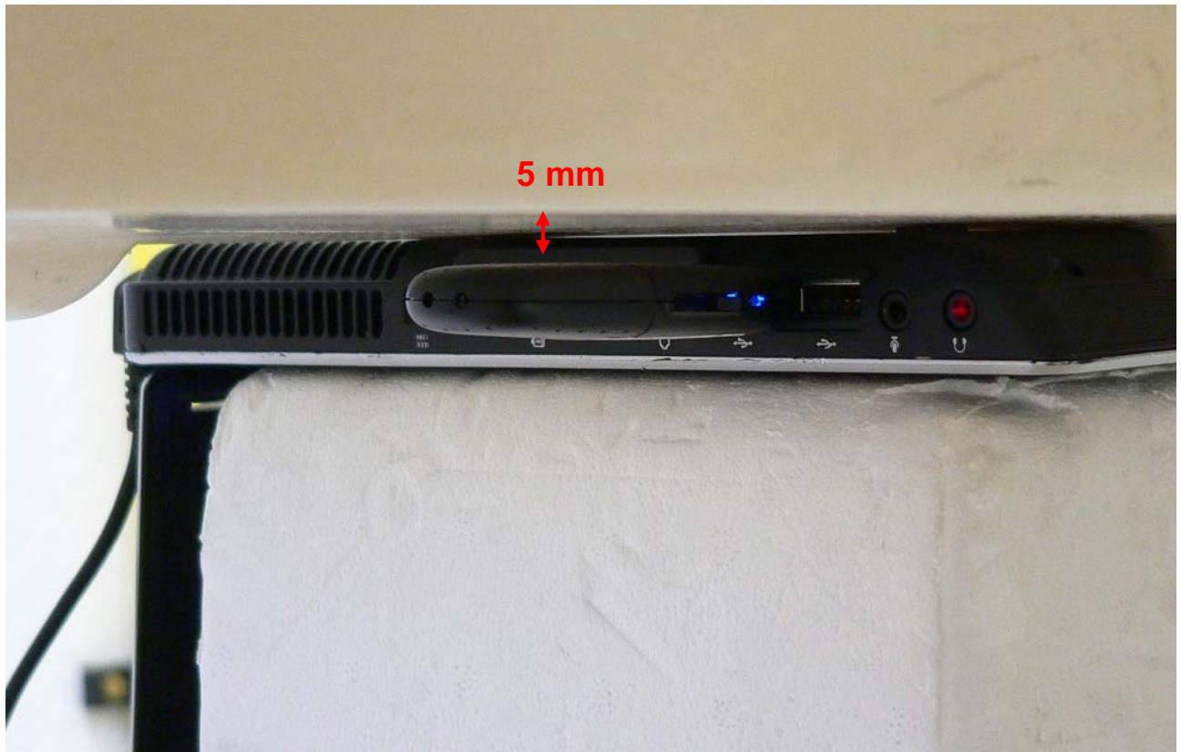
Fig. 16: Position A with the Fujitsu Siemens Amilo Pro.
