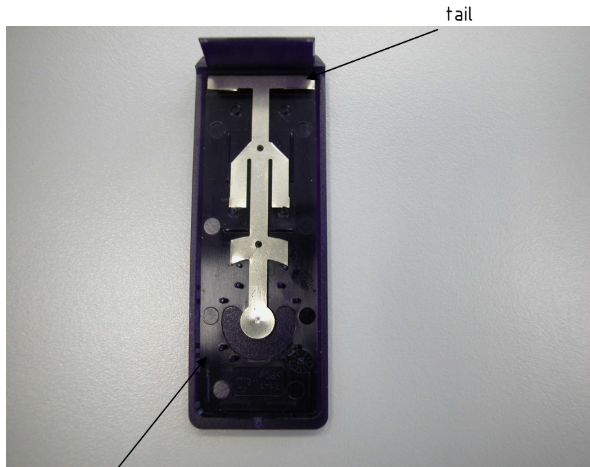
connector (feeding point of the antenna, swivel axis)
