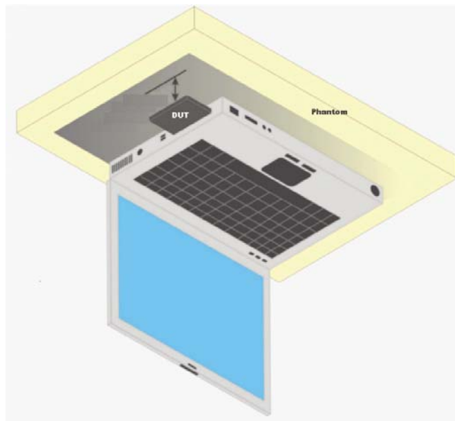
Fig. 6: Lap-held position, bottom of the computer is touching the phantom.
