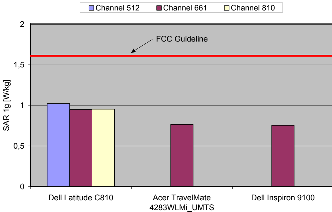
Fig. 10: The measured SAR values for the Option ICONII lite for GPRS 1900 (Class 12) in comparison to the FCC exposure limit.
