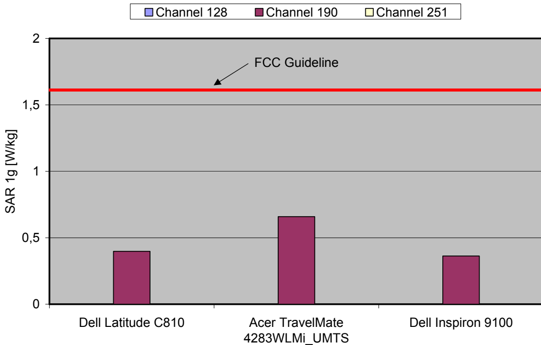
Fig. 9: The measured SAR values for the Option ICONII lite for GPRS 850 (Class 11) in comparison to the FCC exposure limit.
