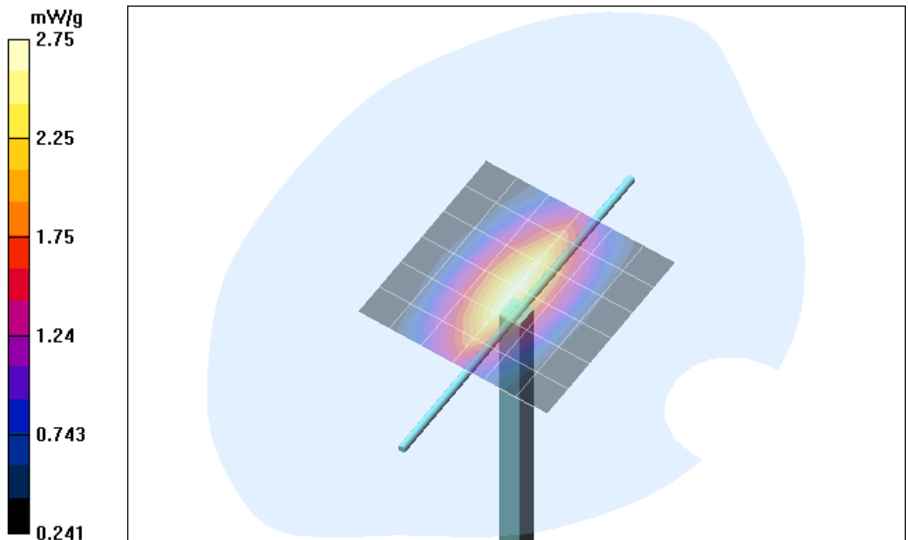
Fig. 11: Validation measurement 835 MHz Body (GSM 850, April 16, 2007), coarse grid. Ambient Temperature: 22.6°C, Liquid Temperature: 21.3°C.
