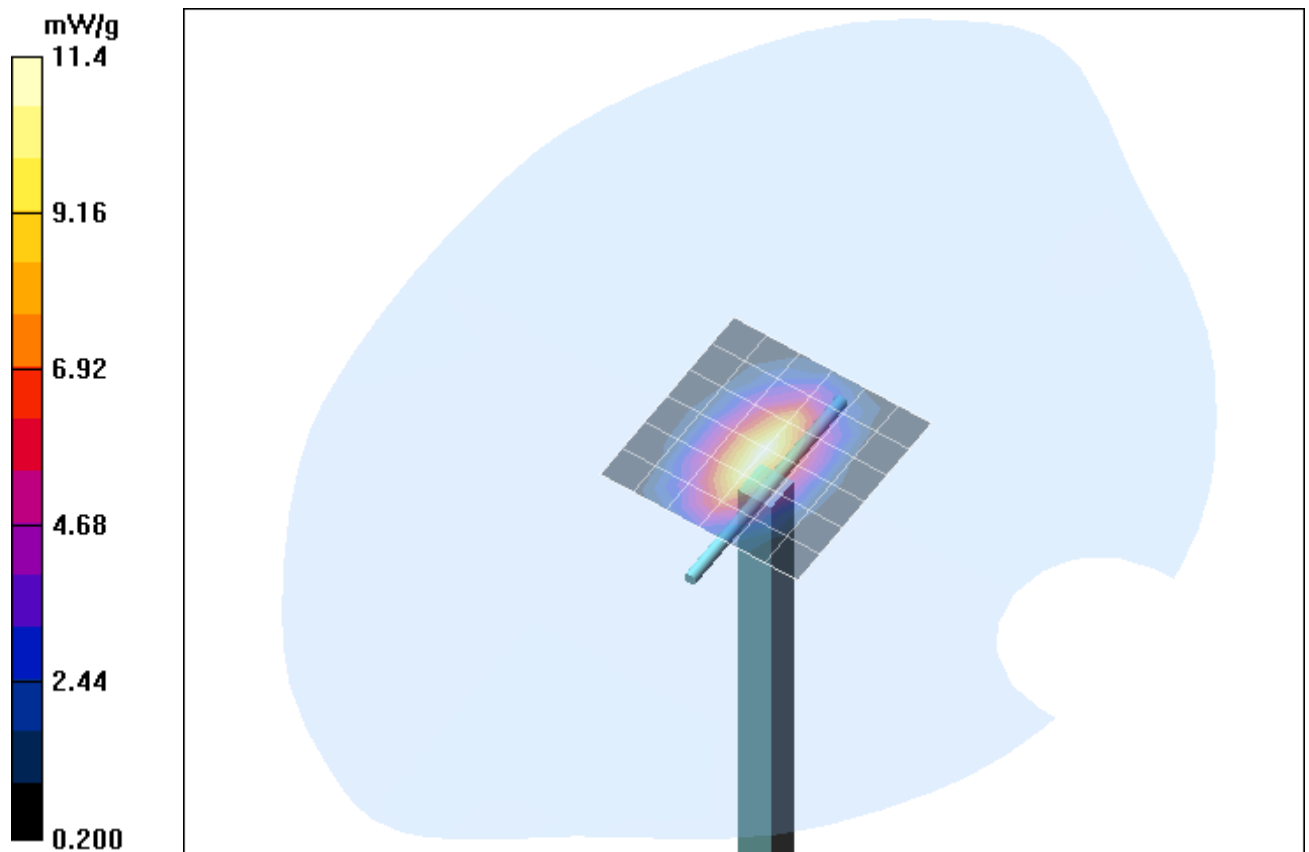
Fig. 12: Validation measurement 1900 MHz Body (GSM 1900, April 17, 2007), coarse grid. Ambient Temperature: 22.7°C, Liquid Temperature: 21.4°C.
