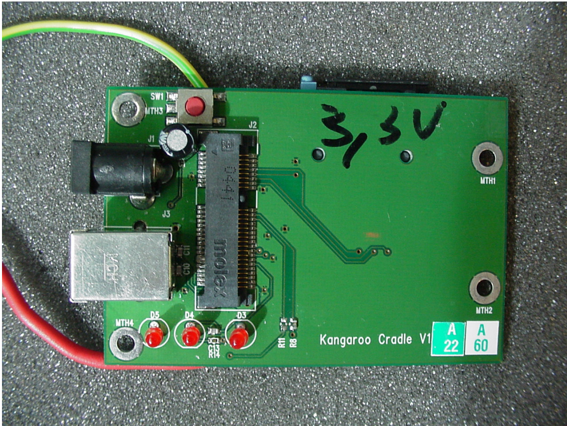
Photo 9: Cradle AE1 (front side)
