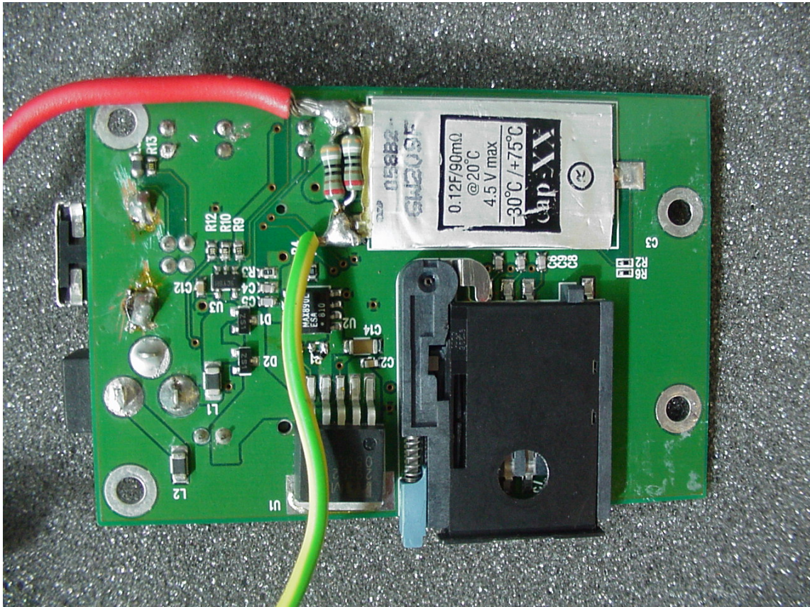
Photo 10: Cradle AE1 (rear side)
