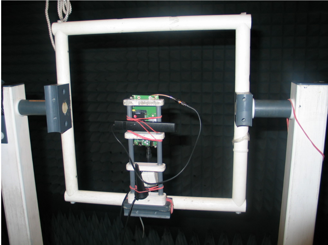
Photo 8: Setup for radiated tests (EUT B operated in a cradle and with external antenna)
