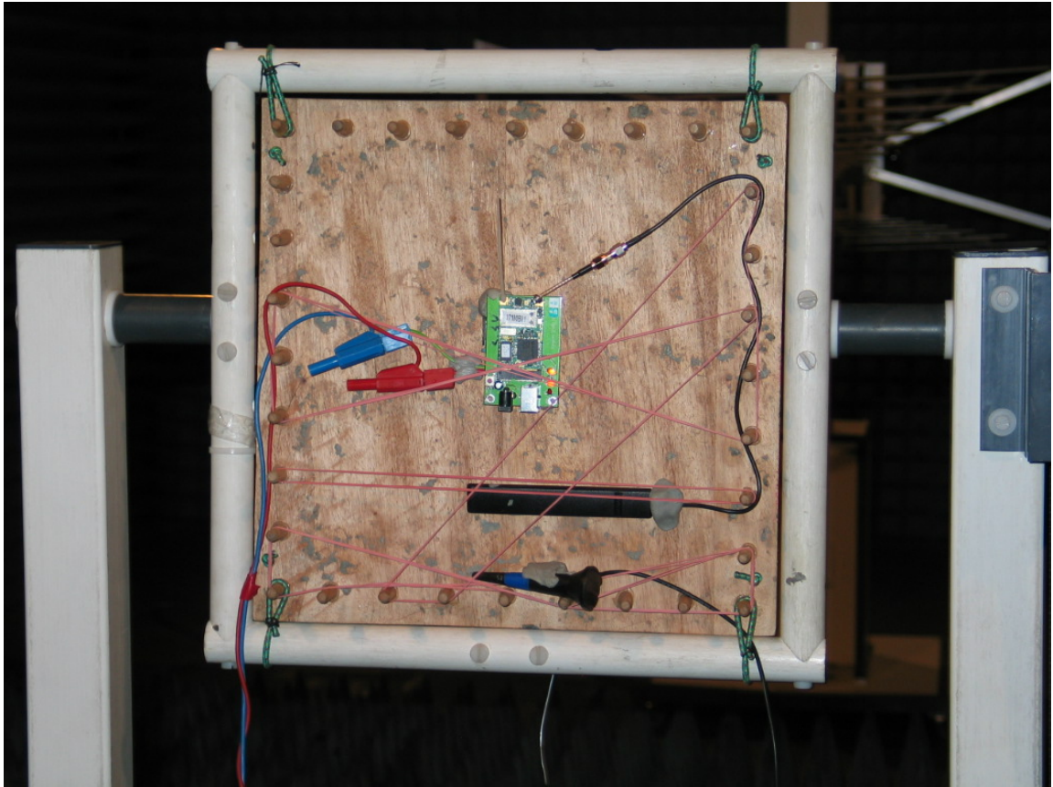
Photo 7: Setup for radiated tests (EUT A operated in a cradle and with external antenna)
