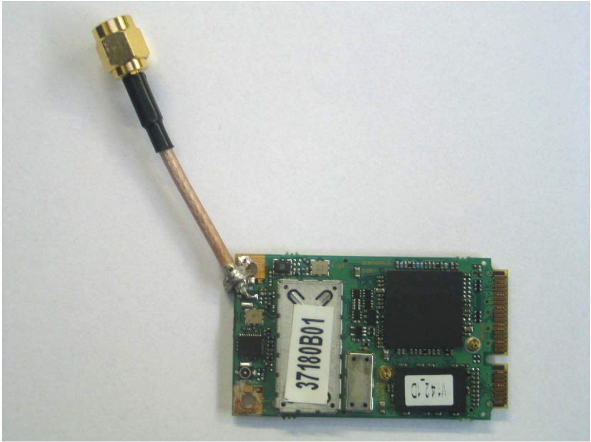
Photo 3: GSM/UMTS module MO201 (front side)
