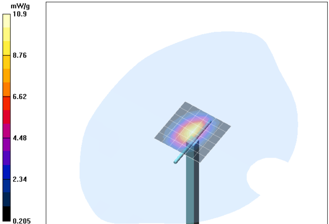
Fig. 16: Validation measurement 1900 MHz Body (WCDMA II, March 29, 2007), coarse grid. Ambient Temperature: 22.4°C, Liquid Temperature: 21.3°C.
