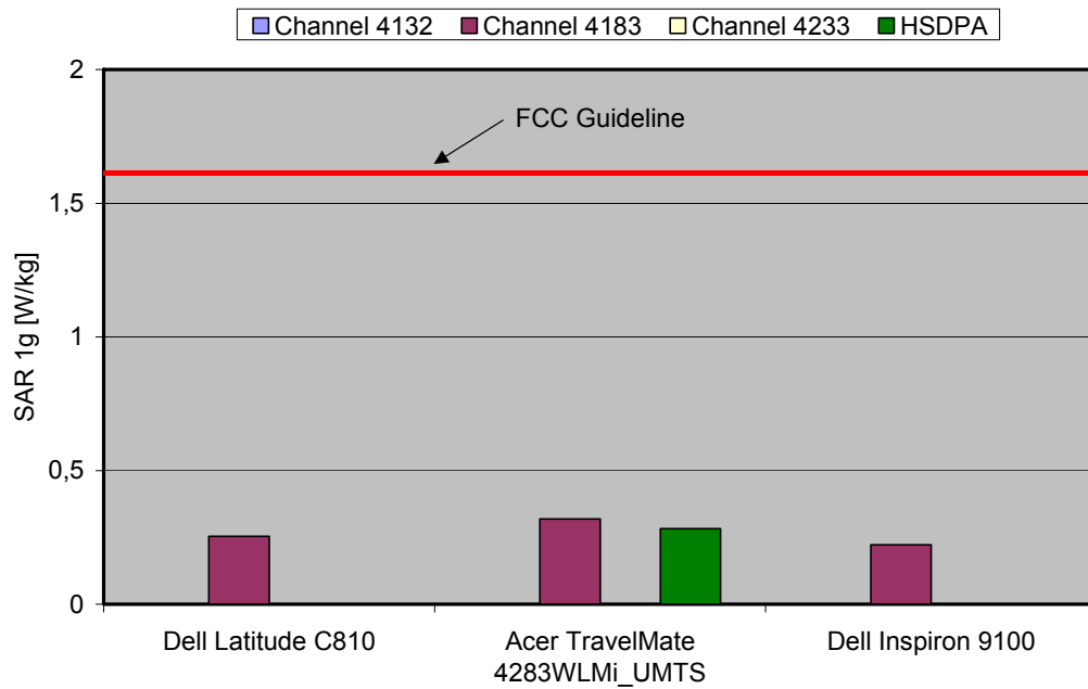
Fig. 12: The measured SAR values for the Option ICONII for WCDMA V (FDD) in comparison to the FCC exposure limit.
