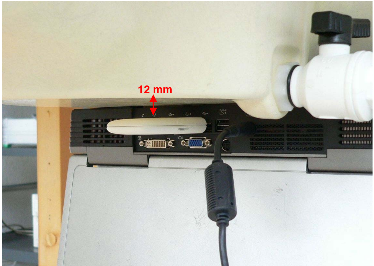
Fig. 27: Lap Held Position with the Dell Inspiron 9100.
