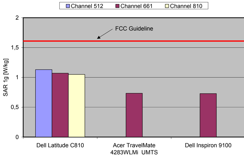
Fig. 10: The measured SAR values for the Option ICONII for GPRS 1900 (Class 12) in comparison to the FCC exposure limit.
