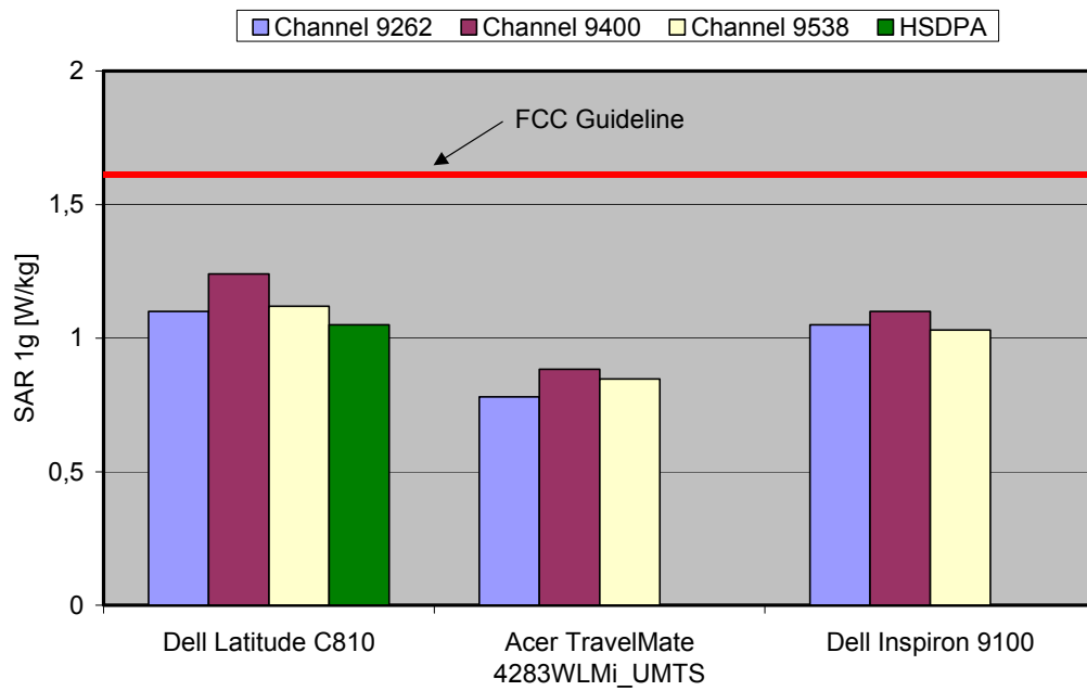
Fig. 11: The measured SAR values for the Option ICONII for WCDMA II (FDD) in comparison to the FCC exposure limit.
