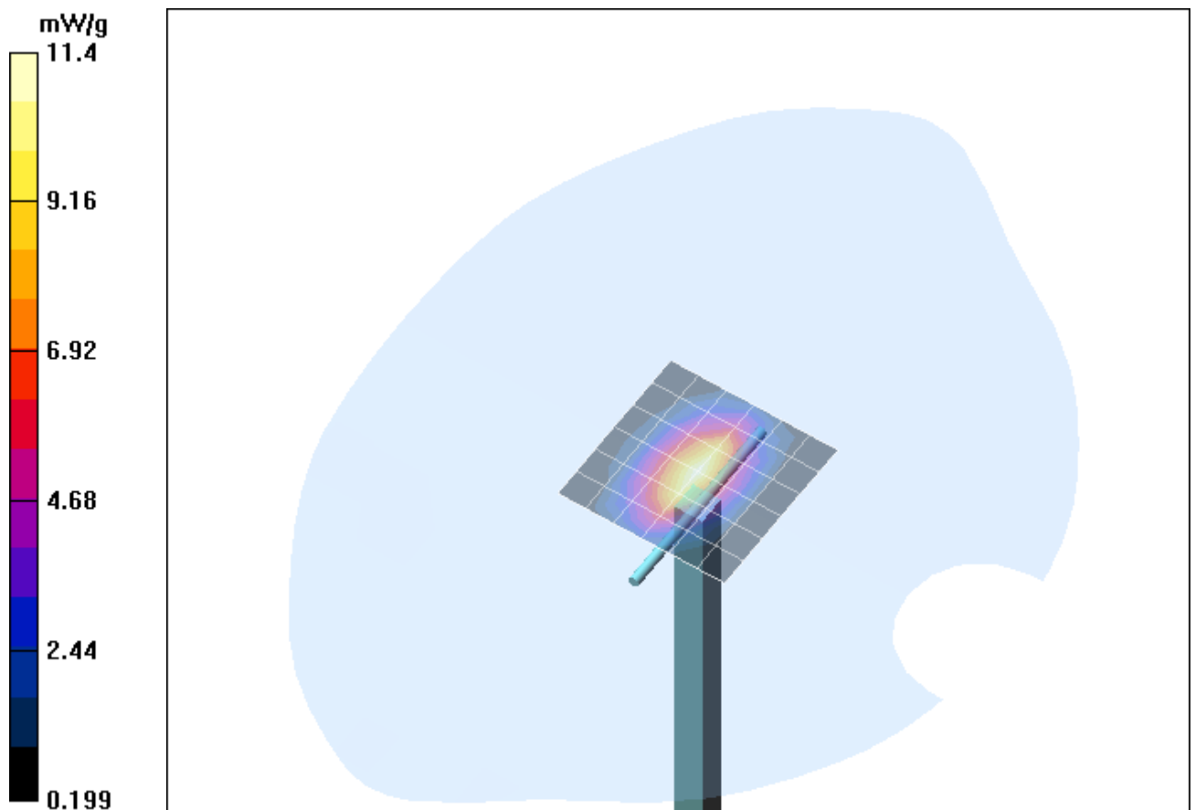
Fig. 15: Validation measurement 1900 MHz Body (GSM 1900, March 28, 2007), coarse grid. Ambient Temperature: 22.1°C, Liquid Temperature: 21.2°C.
