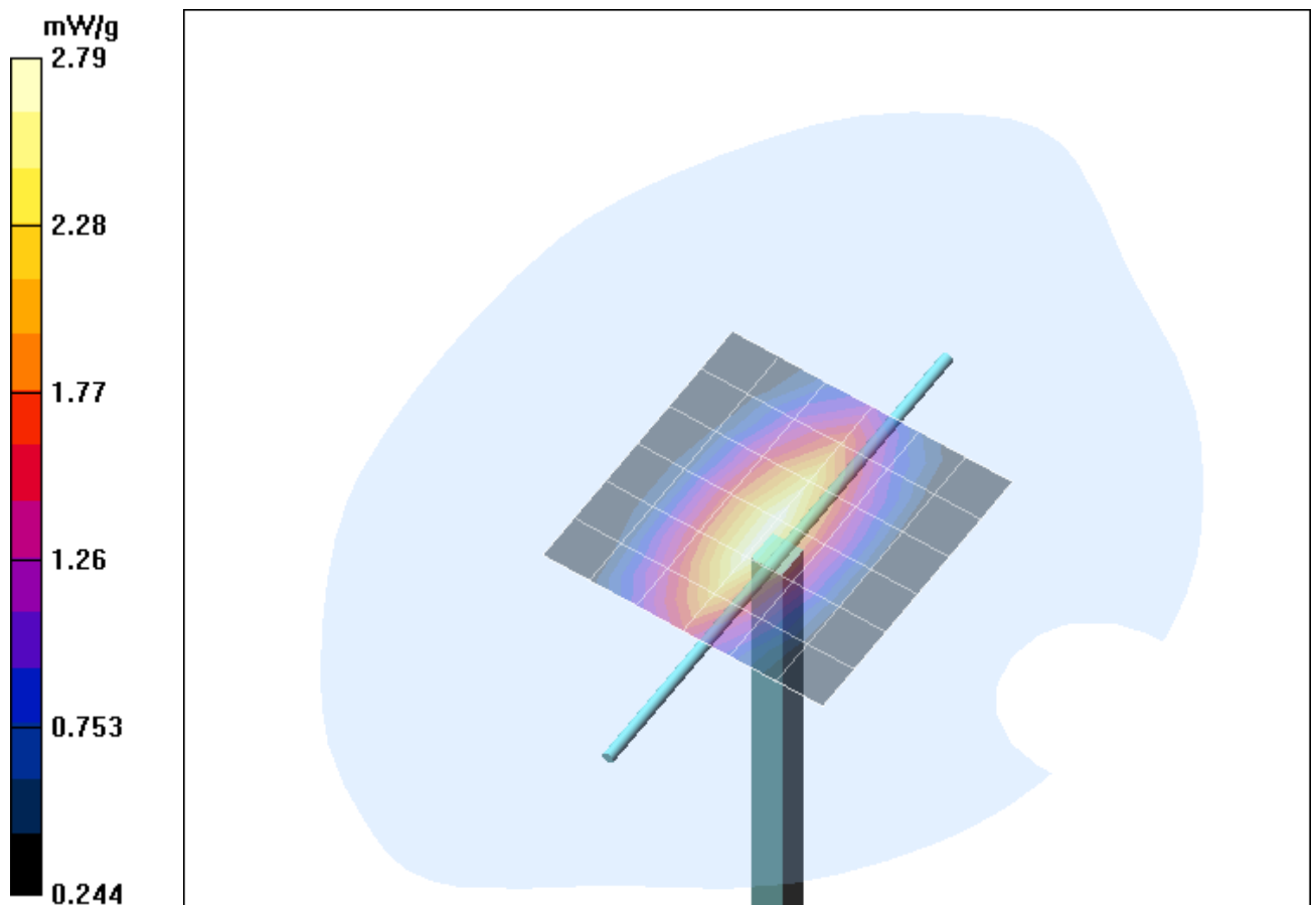
Fig. 14: Validation measurement 835 MHz Body (WCDMA V, March 29, 2007), coarse grid. Ambient Temperature: 22.6°C, Liquid Temperature: 21.5°C.
