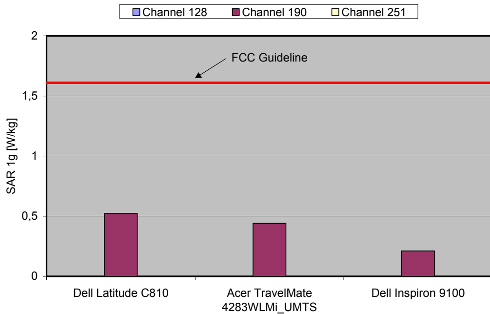
Fig. 9: The measured SAR values for the Option ICONII for GPRS 850 (Class 11) in comparison to the FCC exposure limit.
