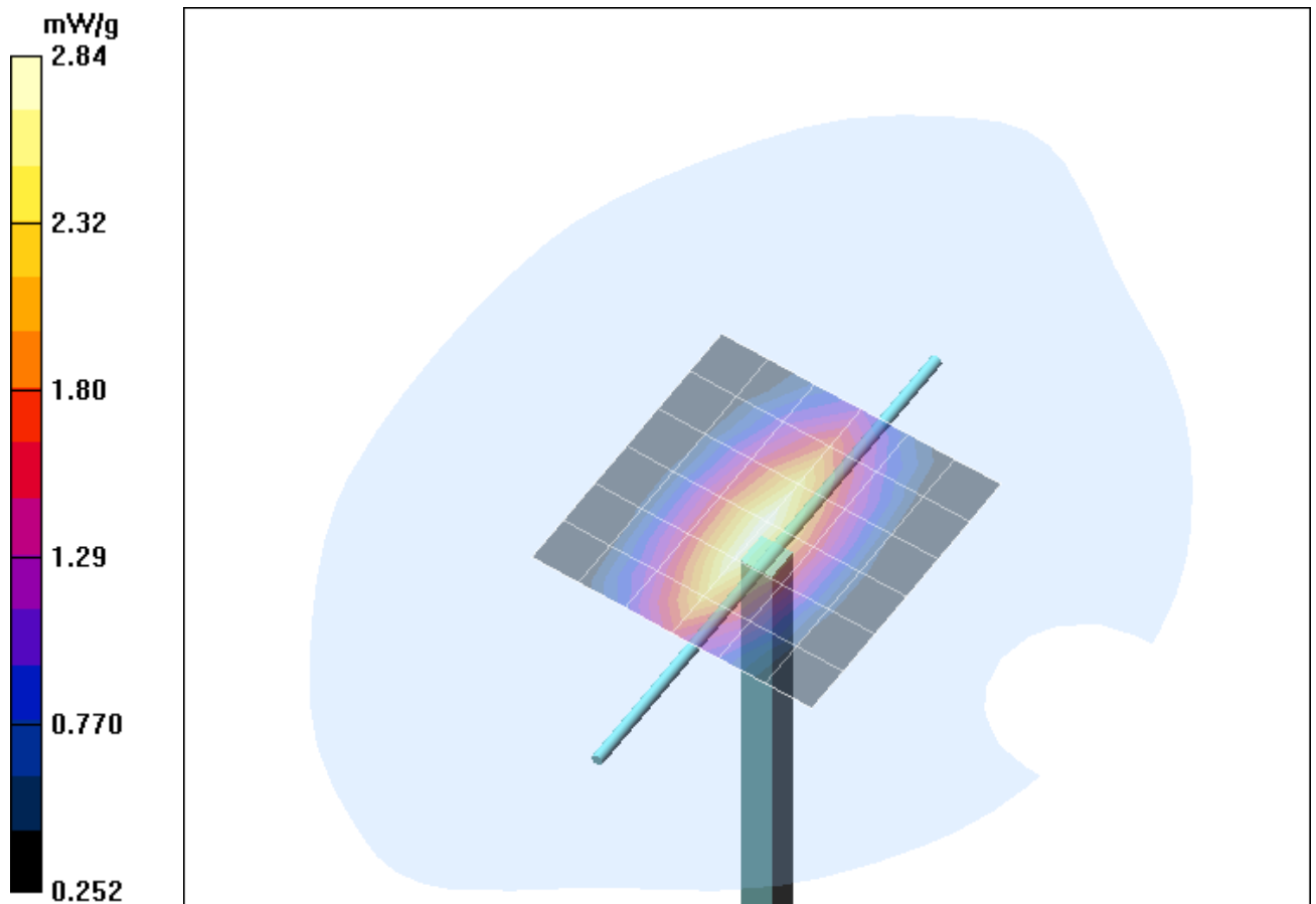
Fig. 13: Validation measurement 835 MHz Body (GSM 850, March 28, 2007), coarse grid. Ambient Temperature: 22.0°C, Liquid Temperature: 21.1°C.
