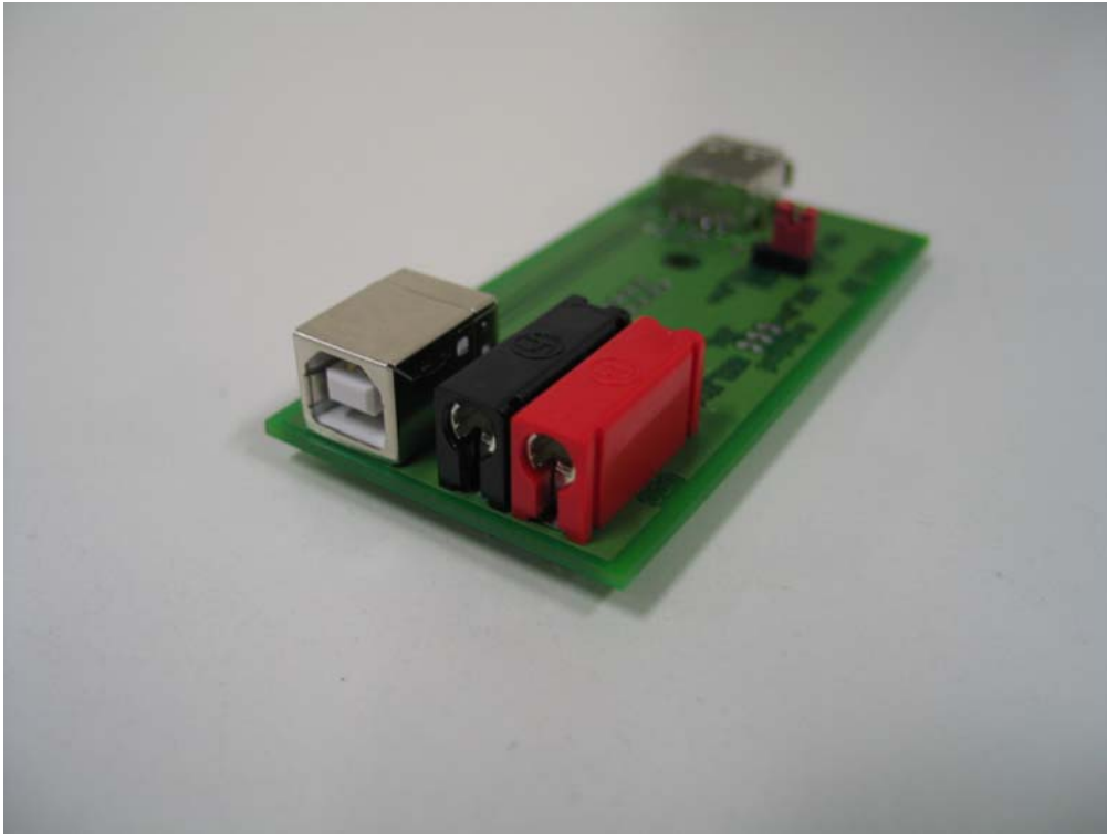
Photo 3: USB Cradle (front side)
