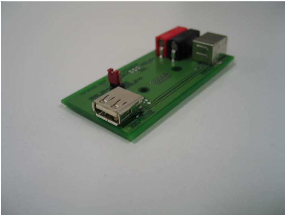
Photo 4: USB Cradle (rear side)
