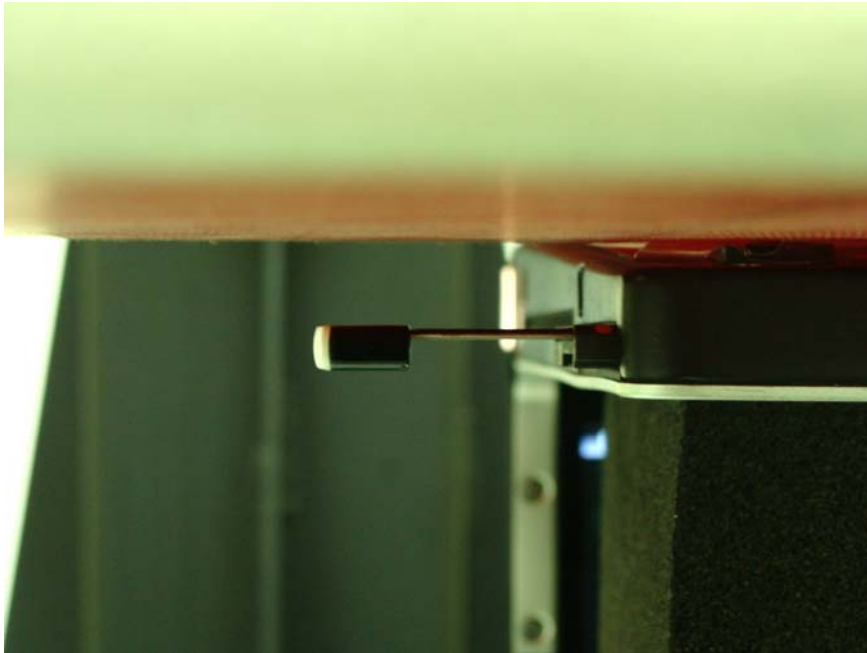
Notebook Bottom Touching Mode with 0 cm Air Gap (Air gap between the DUT and the phantom is 10 mm)
