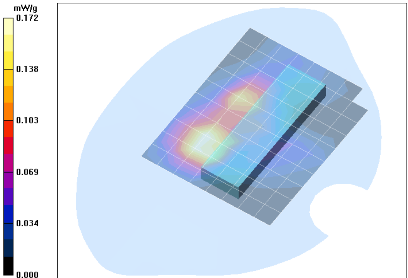
Fig. 10: SAR distribution for WCDMA II (FDD), HSDPA, channel 9400, Lap Held Position (Acer TravelMate, April 02, 2007; Ambient Temperature: 22.1° C; Liquid Temperature: 21.0° C).
