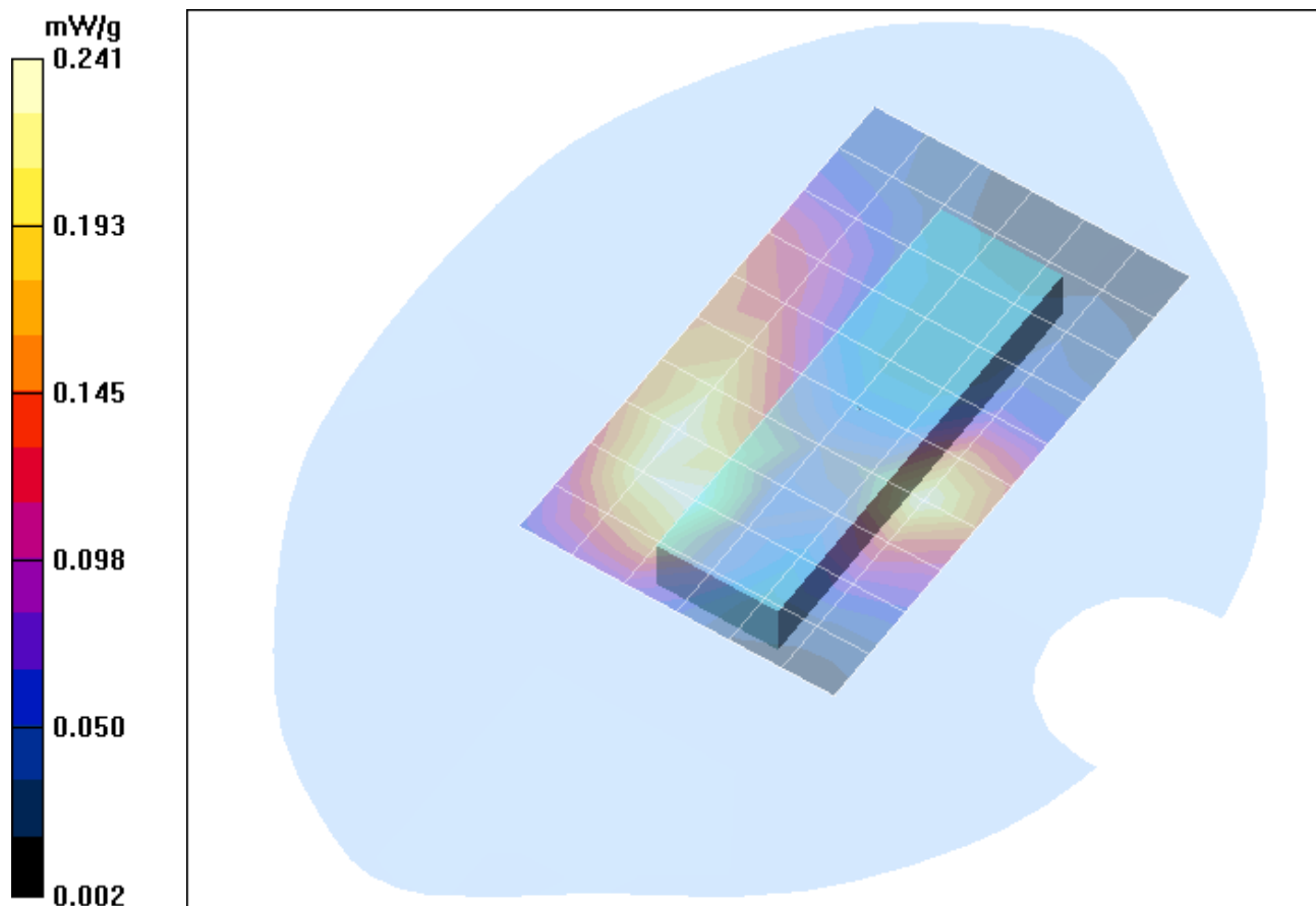
Fig. 6: SAR distribution for GPRS 1900 (Class 12), channel 661, Lap Held Position (HP Compaq nc6320, March 28, 2007; Ambient Temperature: 22.1° C; Liquid Temperature: 21.0C).
