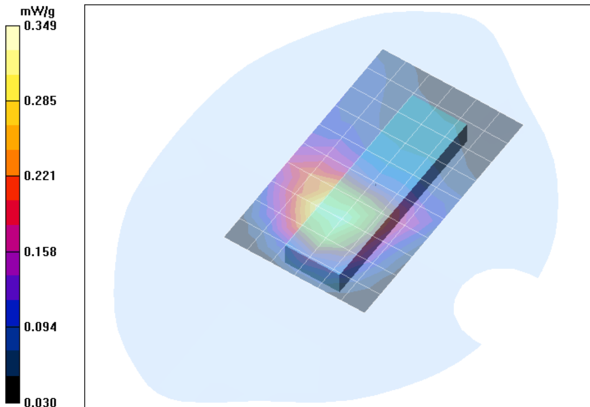
Fig. 14: SAR distribution for WCDMA V (FDD), HSDPA, channel 4183, Lap Held Position (HP Compaq nc6320, March 29, 2007; Ambient Temperature: 22.0° C; Liquid Temperature: 21.0° C).
