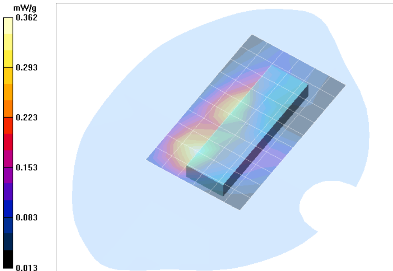
Fig. 5: SAR distribution for GPRS 1900 (Class 12), channel 661, Lap Held Position (Acer TravelMate, March 28, 2007; Ambient Temperature: 22.1° C; Liquid Temperature: 21.3 C).
