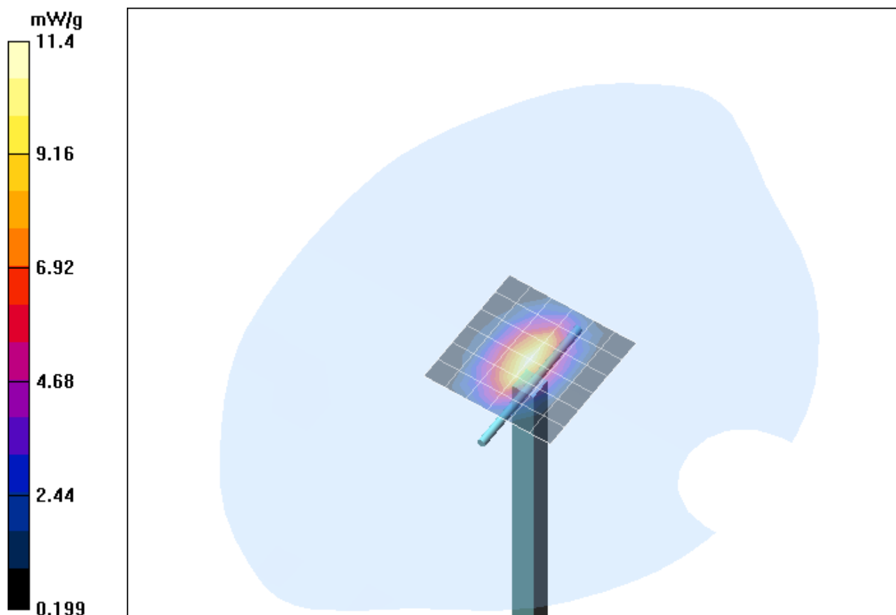
Fig. 14: Validation measurement 1900 MHz Body (GSM 1900, March 28, 2007), coarse grid. Ambient Temperature: 22.1°C, Liquid Temperature: 21.2°C.
