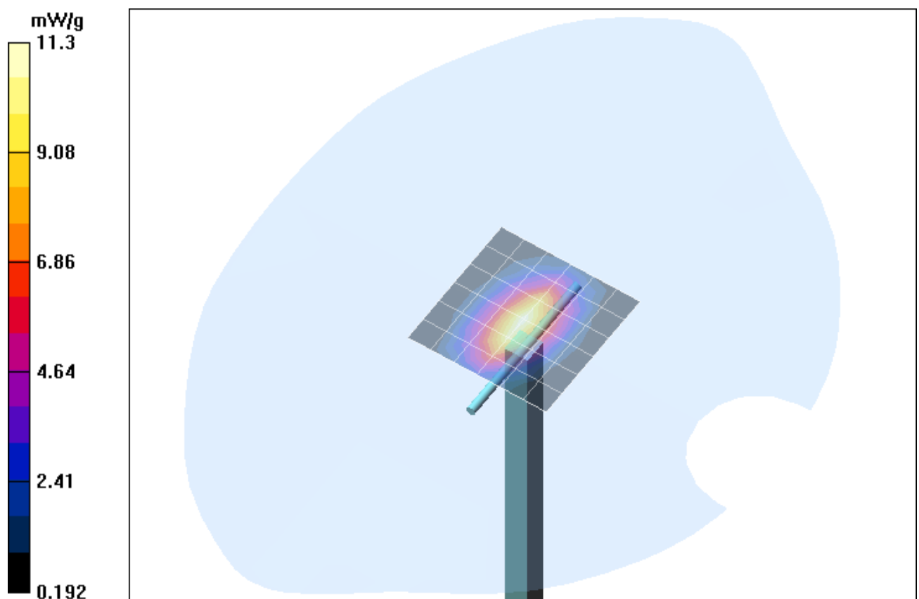
Fig. 18: Validation measurement 1900 MHz Body (GSM 1900, May 03, 2007), coarse grid. Ambient Temperature: 22.0°C, Liquid Temperature: 21.2°C.
