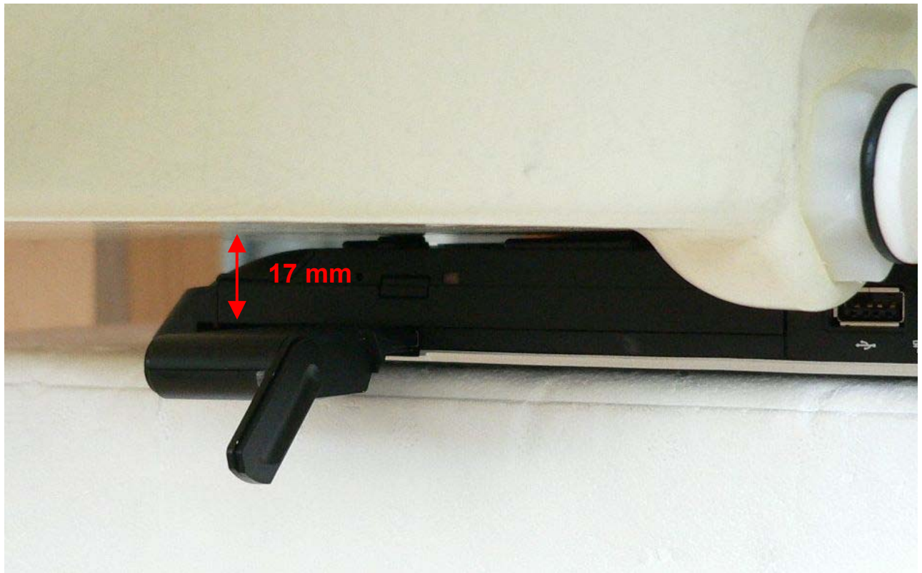
Fig. 24: Lap Held Position with the Fujitsu Siemens AMILO Pro V3205 Notebook, antenna in intended use position.
