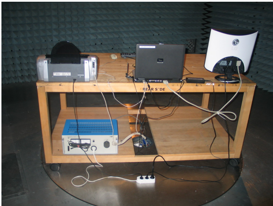
Photo 2: Test setup for radiated measurements (rear side)
