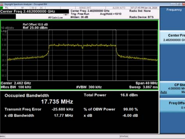
6dB Bandwidth-802.11n(HT20),2462MHz
