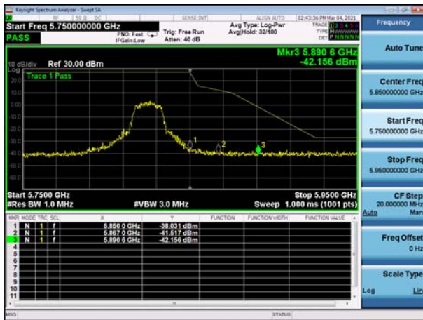
U-NII-3 ,Plot 1,Band Edge-802.11a(20M Hz),5825MHz
