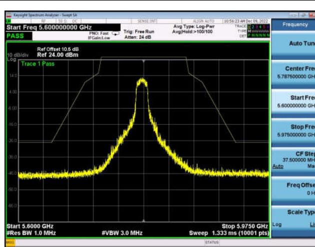
U-NII-3 ,Plot 1,Band Edge-802.11a(20M Hz),5785MHz,Ant1
