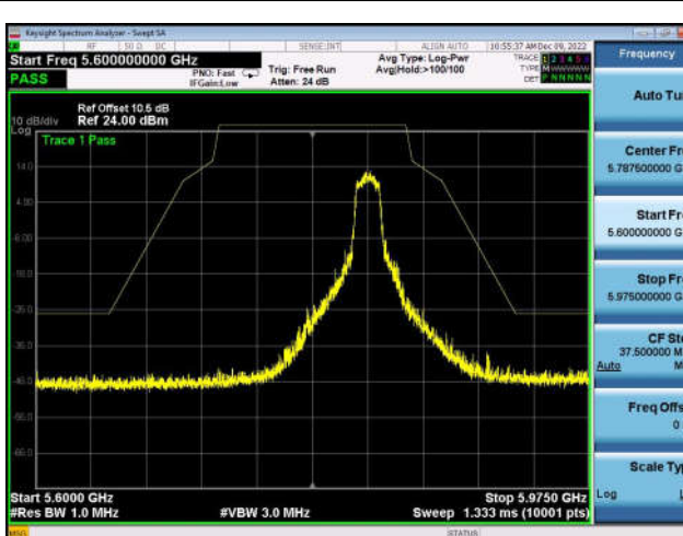
U-NII-3 ,Plot 1,Band Edge-802.11a(20MHz),5825MHz,Ant1
