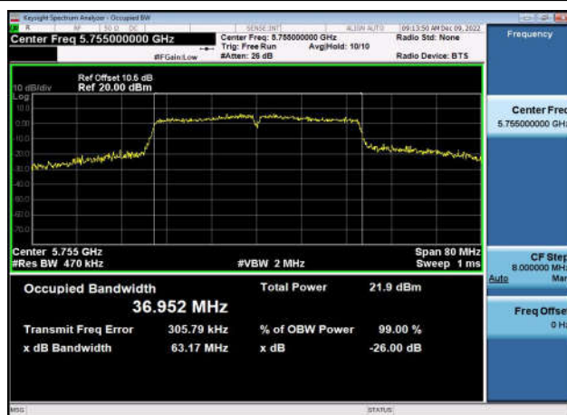
U-NII-3 26dB & 99% Bandwidth-802.11n(40MHz),5755MHz,Ant1
