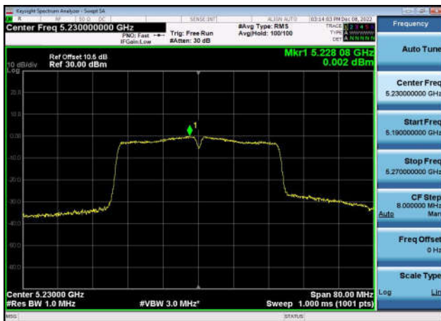
U-NII-1 Power spectral density-802.11 n(40MHz),5230MHz,Ant1
