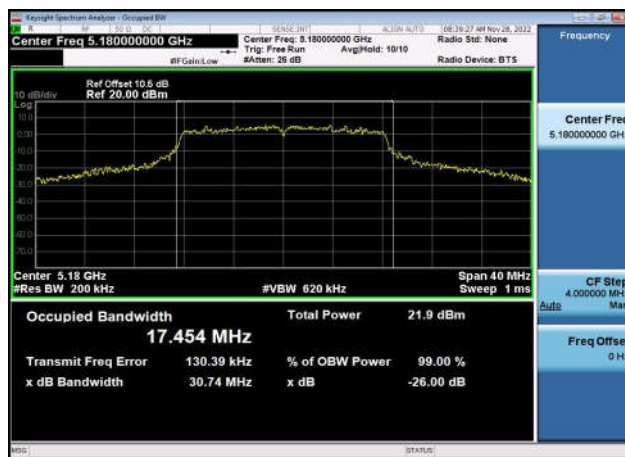
U-NII-1 26dB & 99% Bandwidth-802.11a(20MHz) ,5180MHz,Ant1
