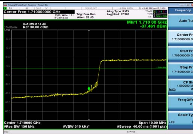
LowRange_FDD66_20MHz_1720_OneRB _low_QPSK
