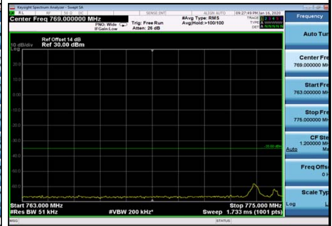
HighRange_FDD13_5MHz_784.5_fullIRB _High_Q16
