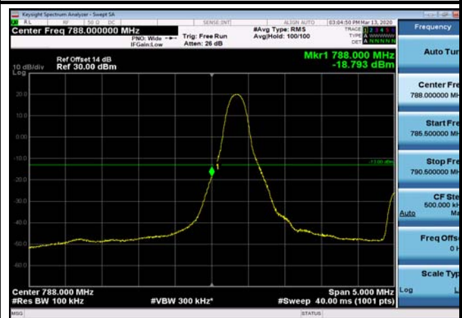
LowRange_FDD14_5MHz_790.5_OneRB _low_Q16
