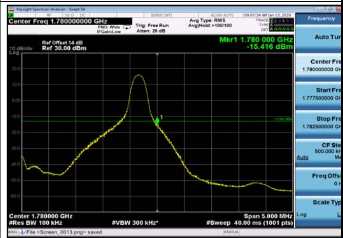
HighRange_FDD66_5MHz_1777.5_OneRB _high_Q16
