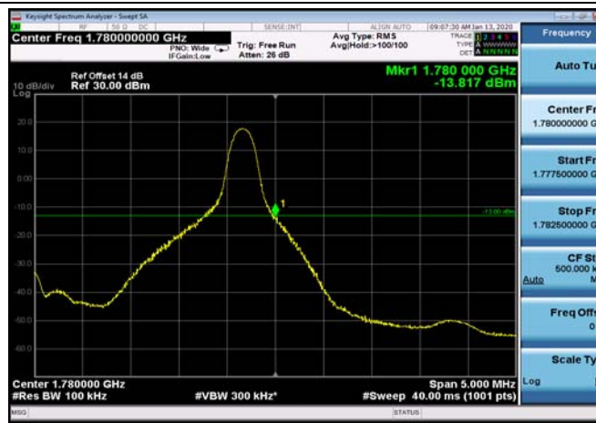
HighRange_FDD66_5MHz_1777.5_OneRB _high_QPSK
