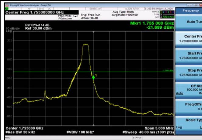
HighRange_FDD04_3MHz_1753.5_fullIRB _High_QPSK
