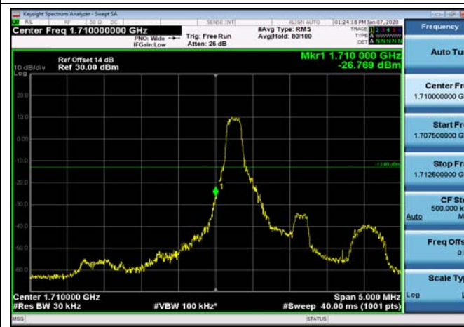
LowRange_FDD66_1.4MHz_1710.7_OneRB _low_QPSK
