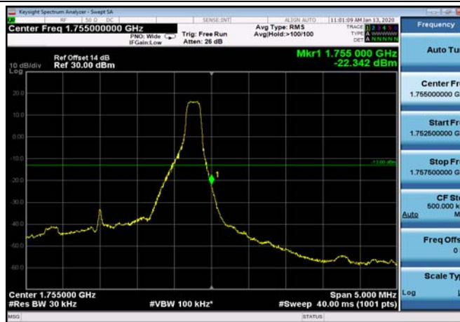
HighRange_FDD04_3MHz_1753.5_fullIRB _High_Q16
