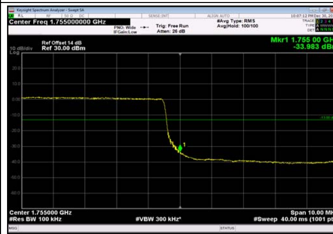
HighRange_FDD04_10MHz_1750_fullIRB _High_QPSK
