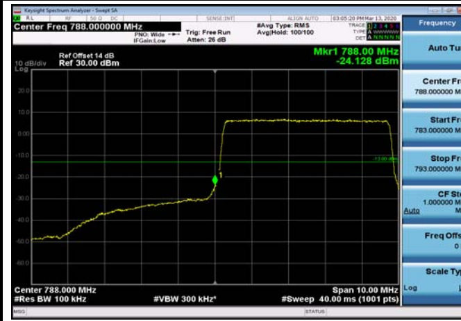
LowRange_FDD14_10MHz_793_OneRB _low_QPSK
