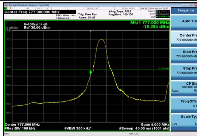
LowRange_FDD13_5MHz_779.5_fullRB_Low_QPSK
