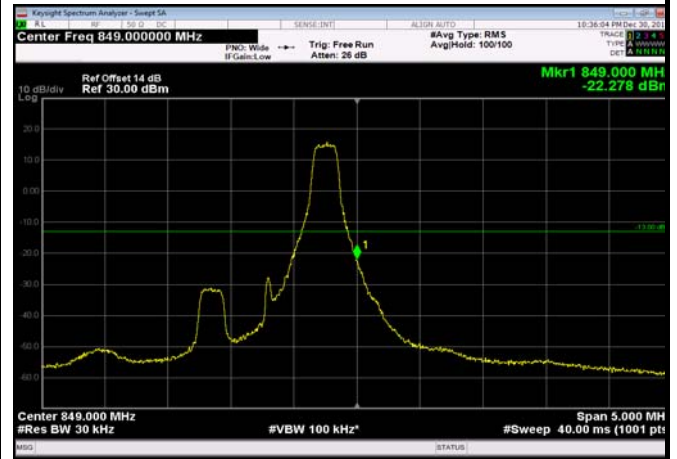
HighRange_FDD05_1.4MHz_848.3_fullIRB _High_Q16
