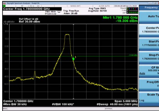
HighRange_FDD66_3MHz_1778.5_fullIRB _High_QPSK
