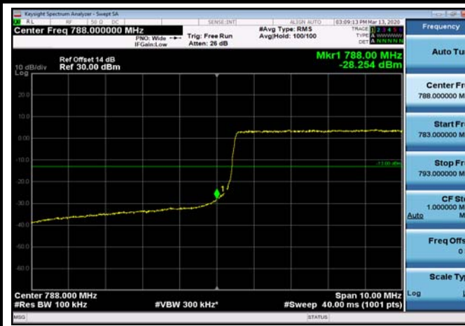
LowRange_FDD14_10MHz_793_fullRB _Low_QPSK
