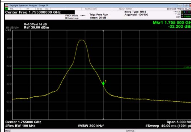
HighRange_FDD04_10MHz_1750_fullIRB _High_QPSK
