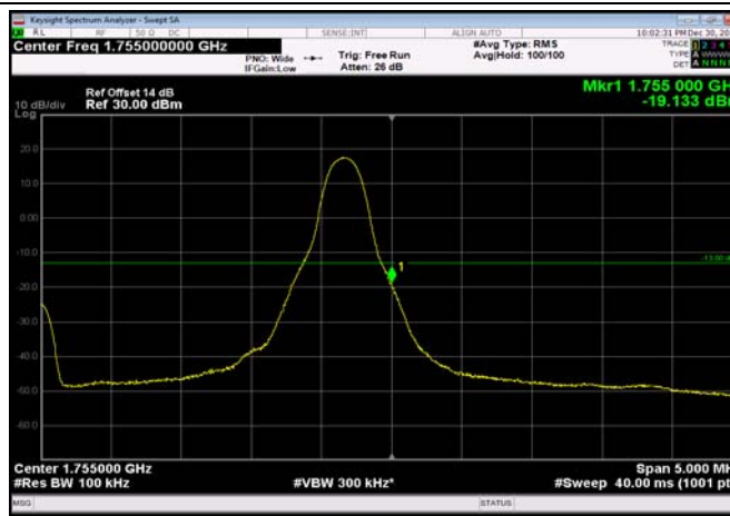
HighRange_FDD04_5MHz_1752.5_OneRB _high_Q16
