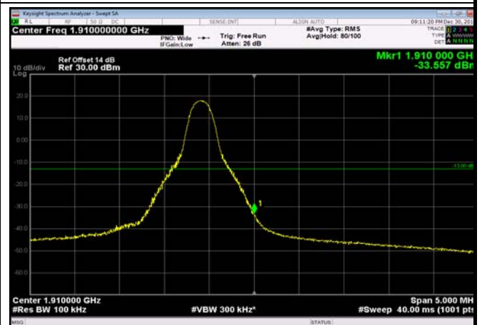
HighRange_ FDD02_10MHz_1905_fullIRB _High_Q16
