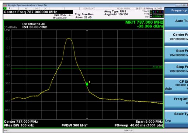
HighRange_FDD13_10MHz_782_OneRB _high_QPSK
