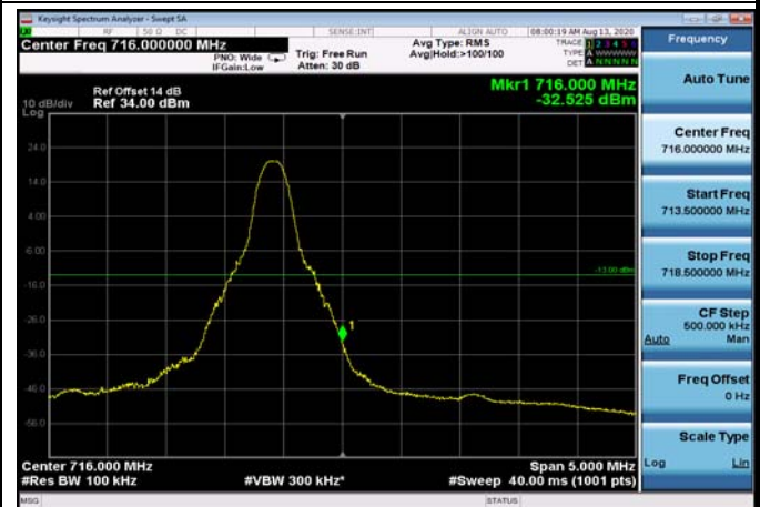
HighRange_FDD12_10MHz_711_OneRB _high_Q16
