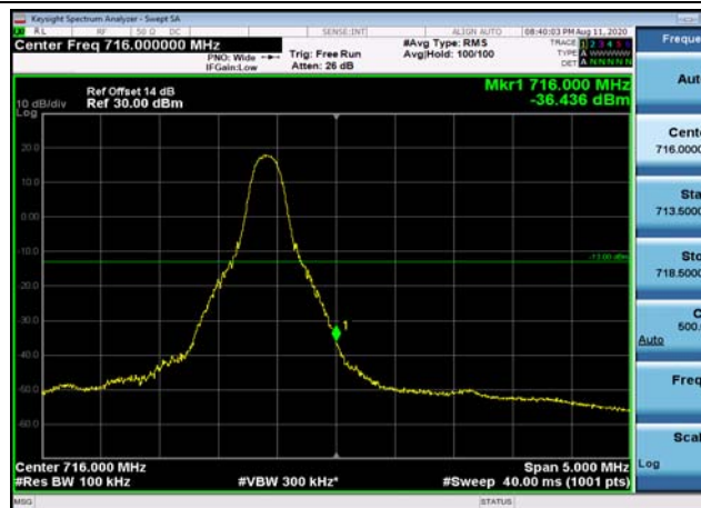
HighRange_FDD12_10MHz_711_OneRB _high_QPSK
