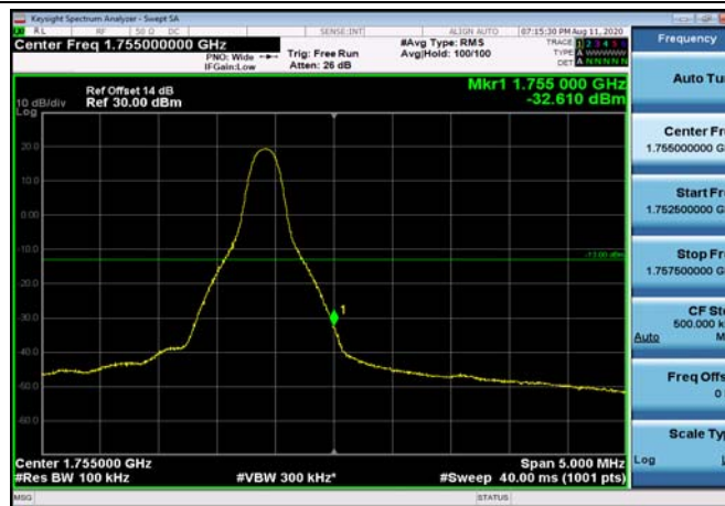
HighRange_FDD04_10MHz_1750_fullIRB _High_QPSK
