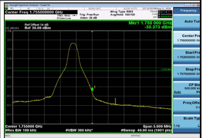
HighRange_FDD04_10MHz_1750_fullIRB _High_Q16
