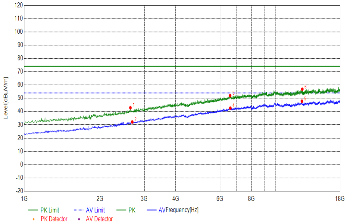
(Plot M: Test Antenna Horizontal 1G – 18G)
