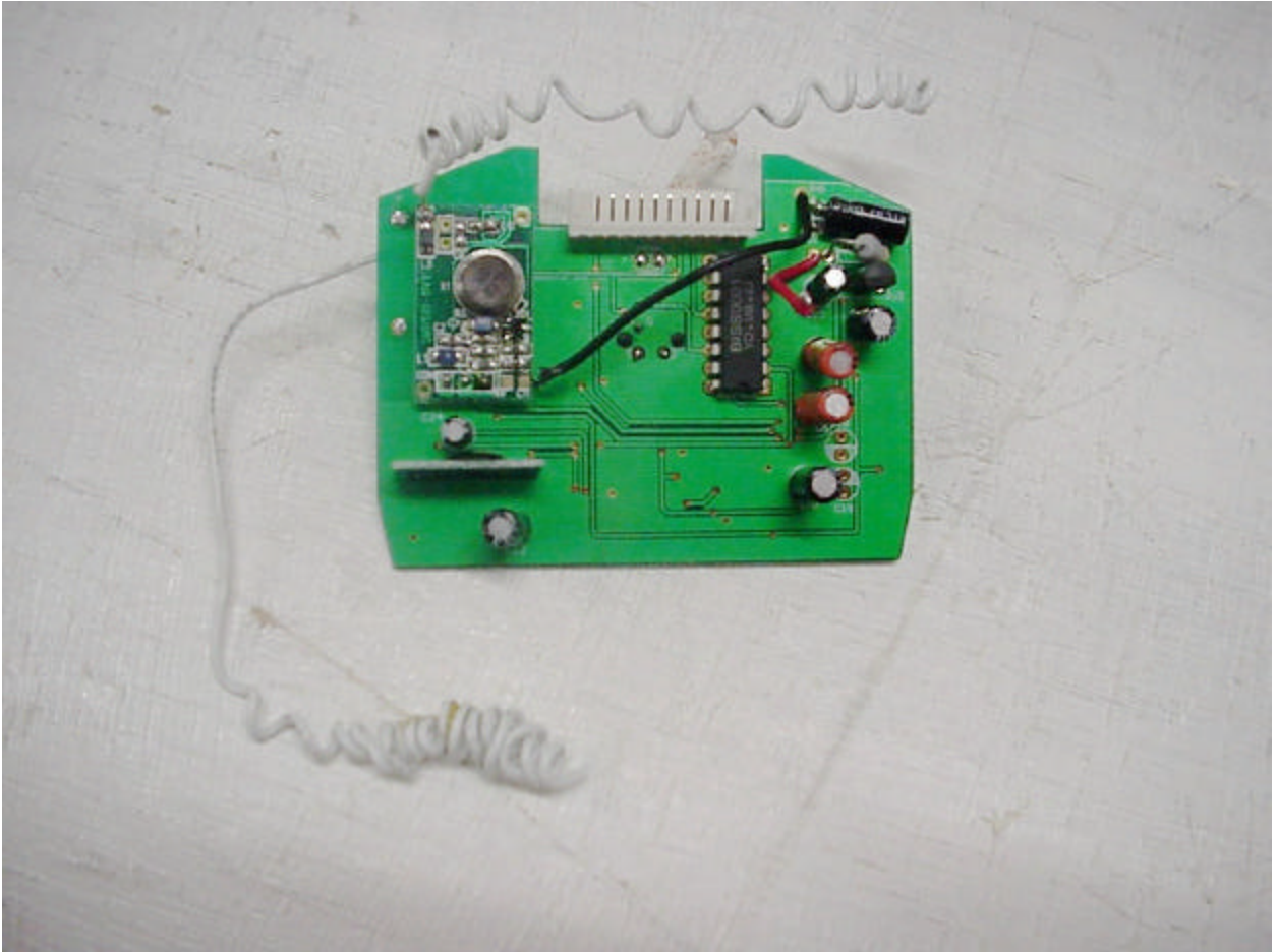
Photo 4. Transmitter Board, Component Side
