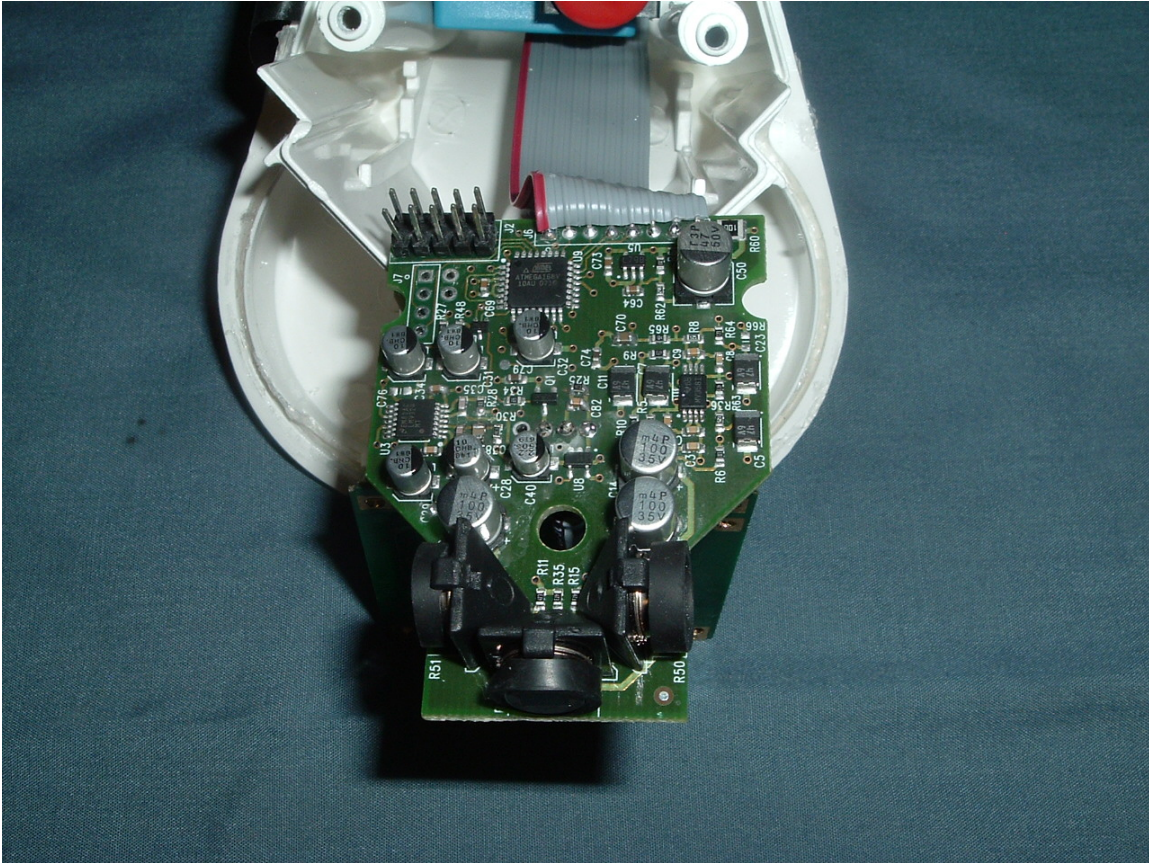
Figure 15. PCB, Component Side.
