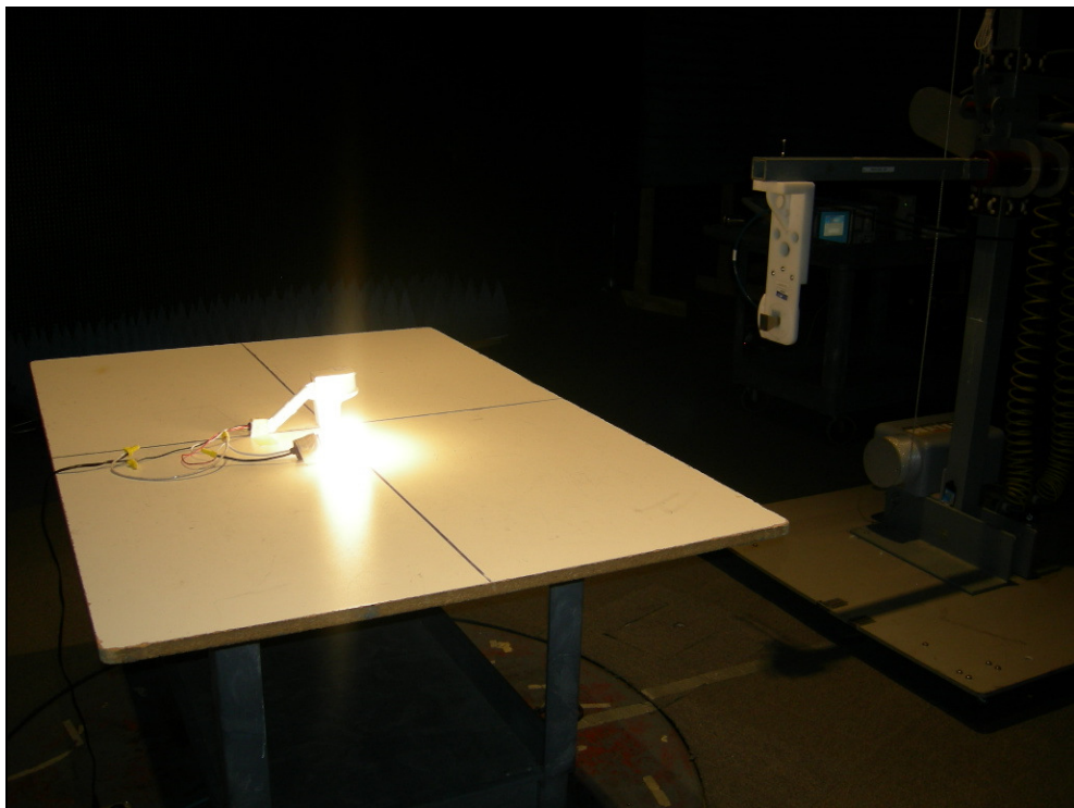
Figure 6: Radiated Emissions
