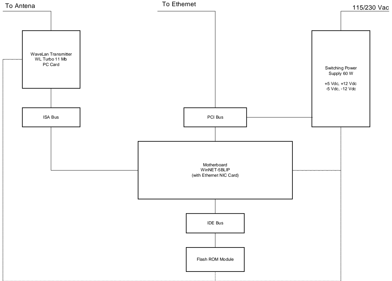
Block Diagram of Wireless Ethernet Bridge NCBSLXE2
