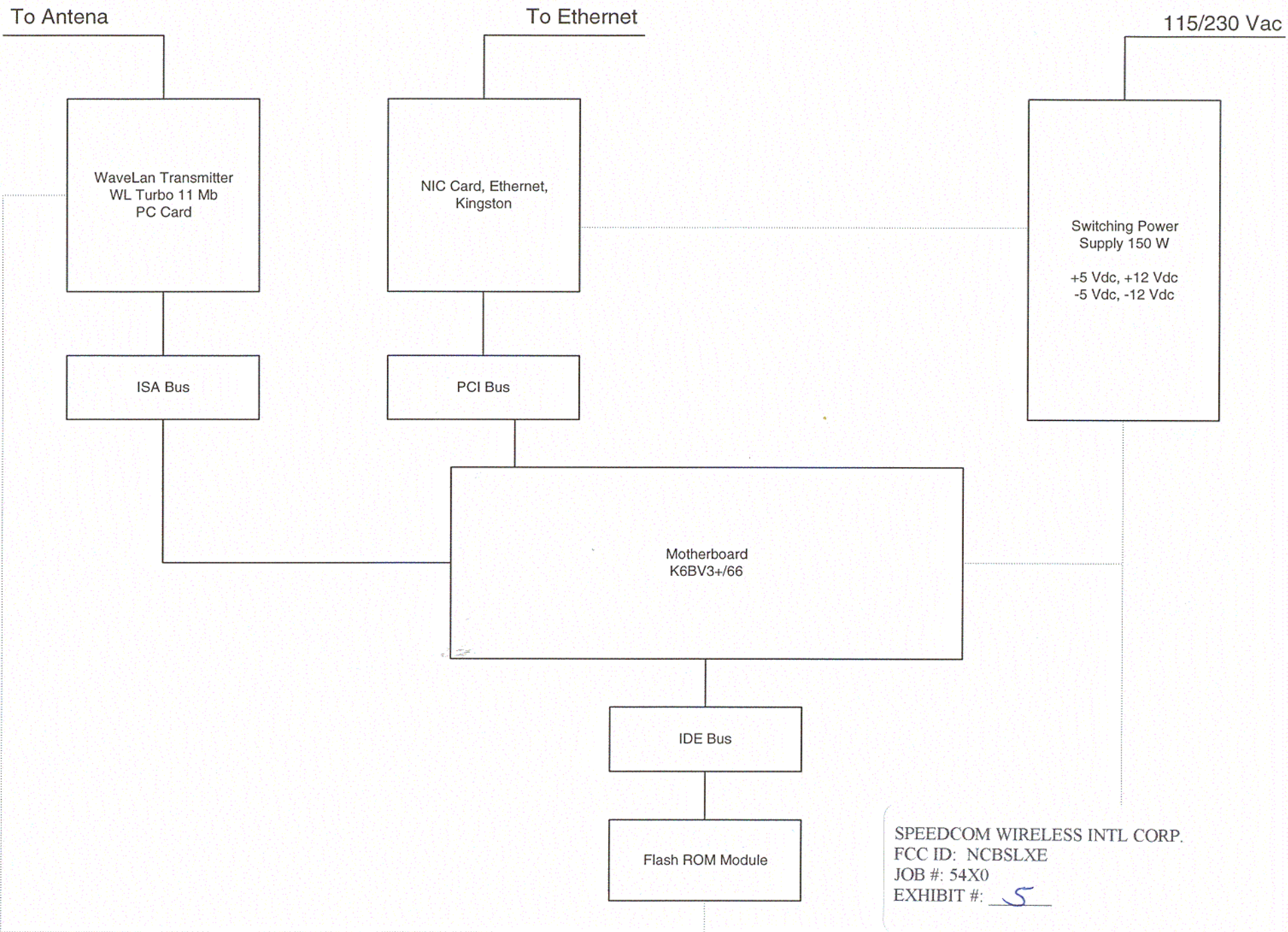
Block Diagram of Wireless Ethernet Bridge NCBSLXE
