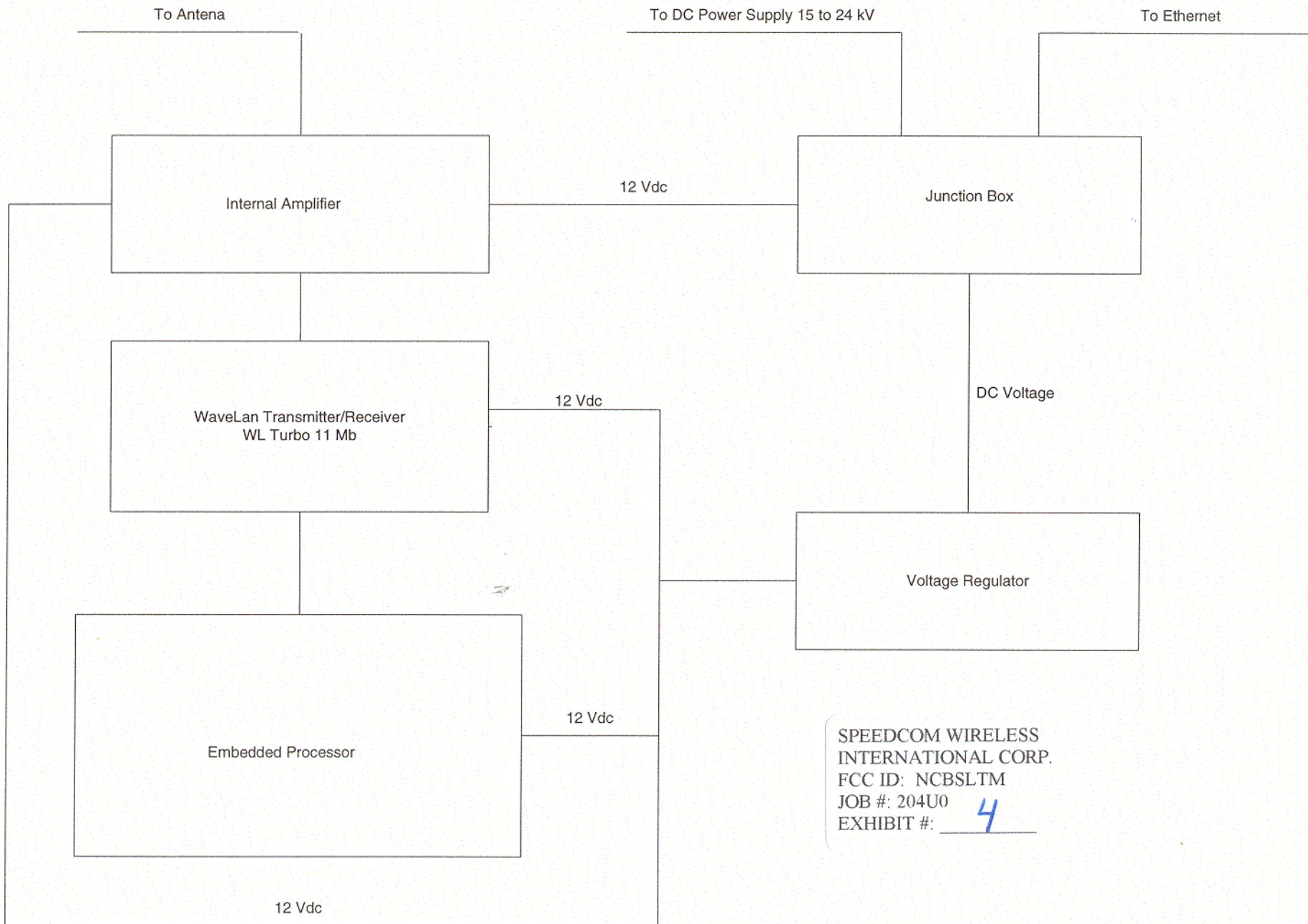
Block Diagram of Wireless Remote Tower Mount Ethernet NCBSLTM Bridge
