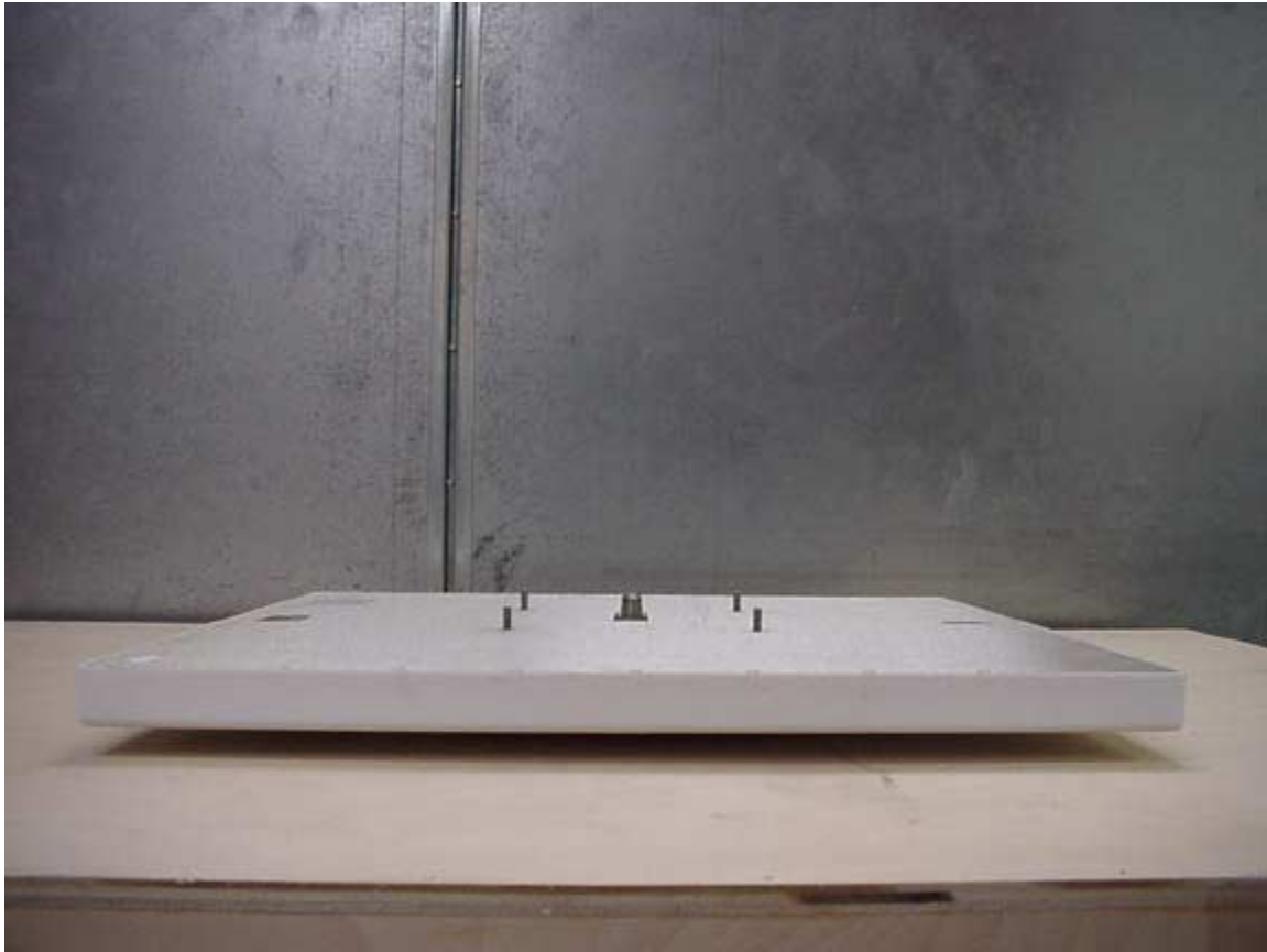
Side of 0.6m Flat Panel Antenna
