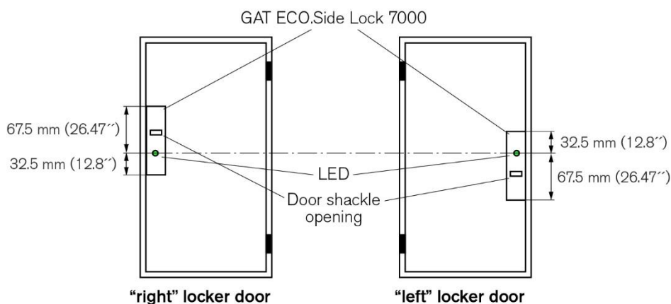
Figure 3.13 - LED positions of the GAT ECO.Side Lock 7000 BA for right and left-hinged doors
