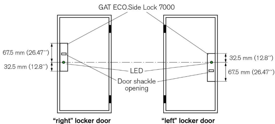
Figure 3.10 - LED positions of the GAT ECO.Side Lock 7000 BA for right and left-hinged doors
