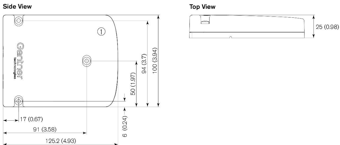
Figure 3.5 - Dimensions of the GAT ECO.Side Lock 7000 BA (dimensions in mm – inches shown in brackets)
