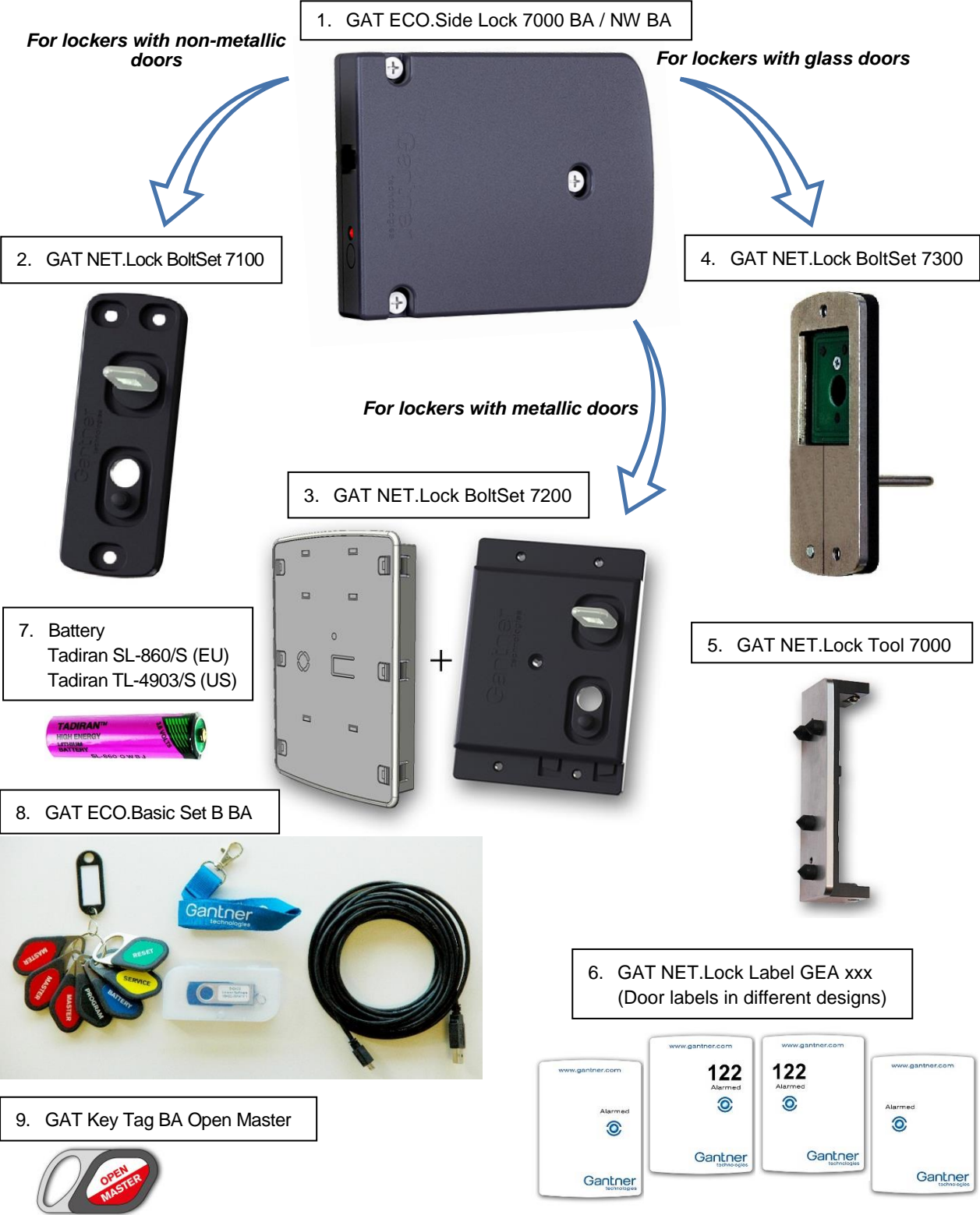
Figure 2.1 – Components of the GAT ECO.Side Lock 7000 system
