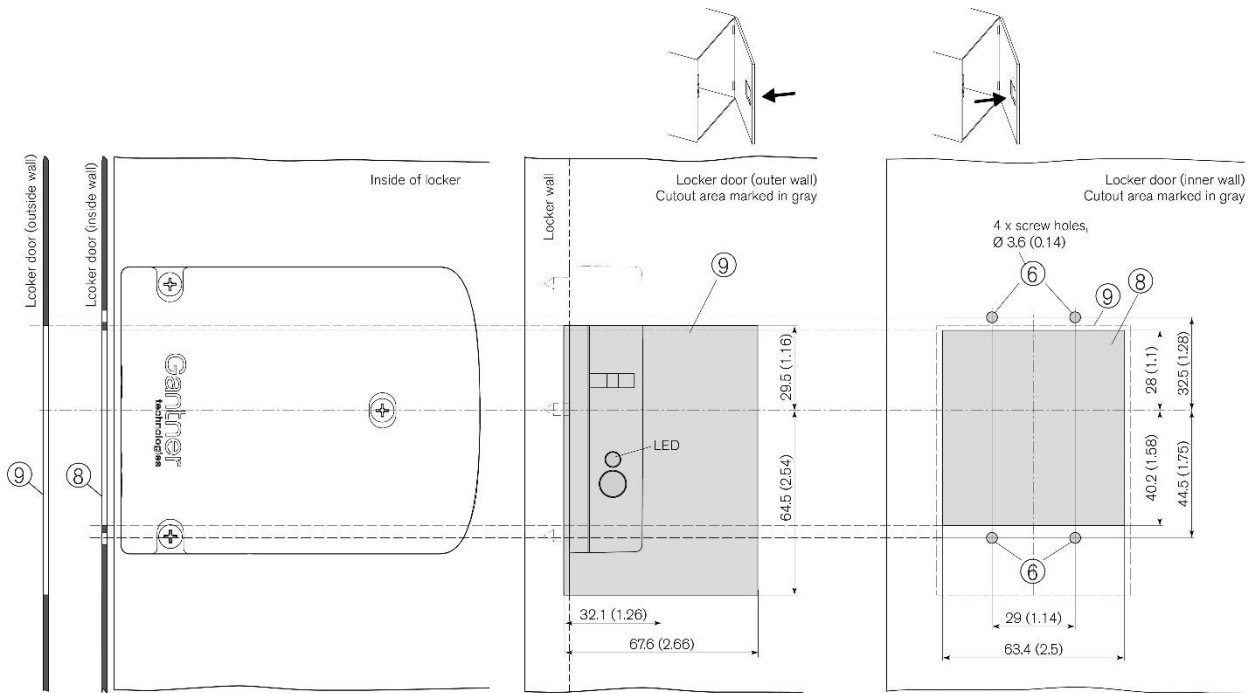
Figure 3.12 - Cutouts for metallic locker doors (dimensions in mm – inches shown in brackets)
