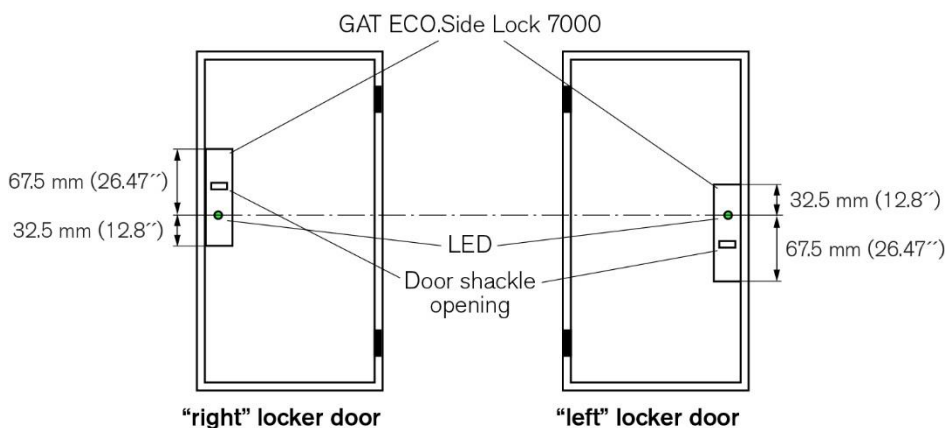
Figure 3.16 - LED positions of the GAT ECO.Side Lock 7000 BA for right and left-hinged doors
