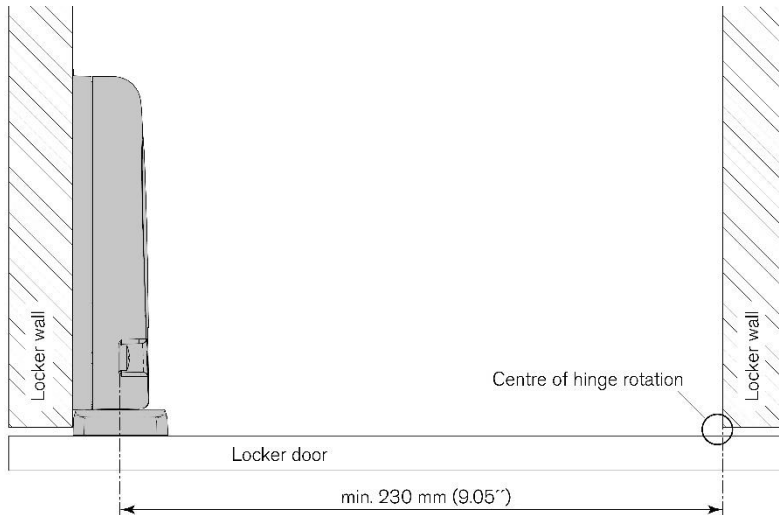
Figure 3.4 - Minimum door width
