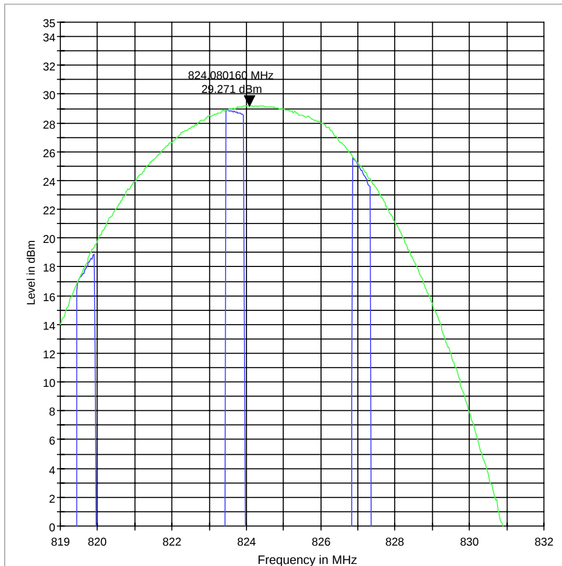
ERP 850 L
