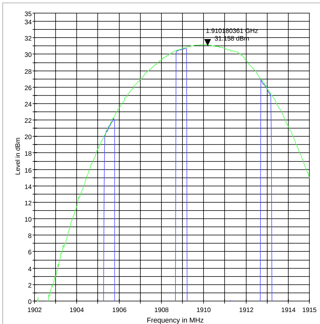
EIRP 1900 H
