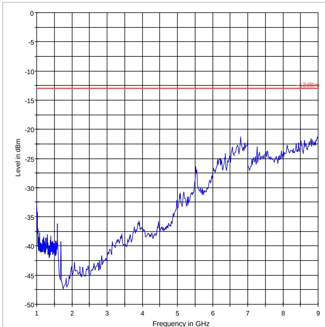
FCC 22 1-9GHz
