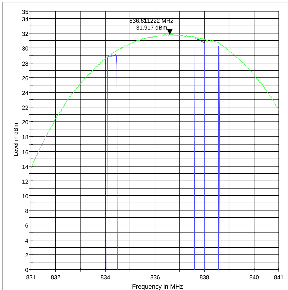
ERP 850 M
