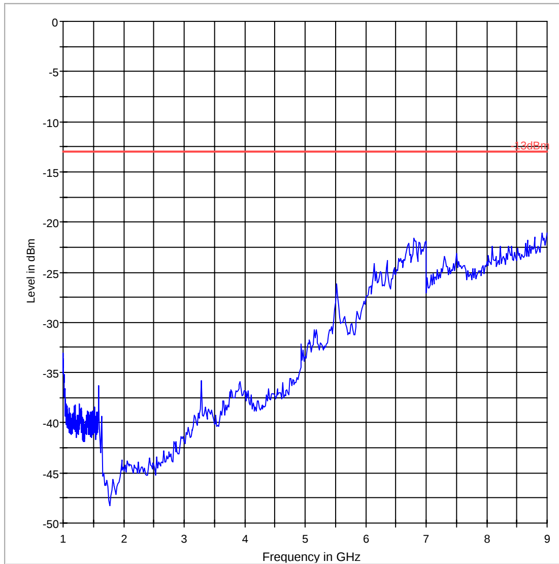
FCC 22 1-9GHz
