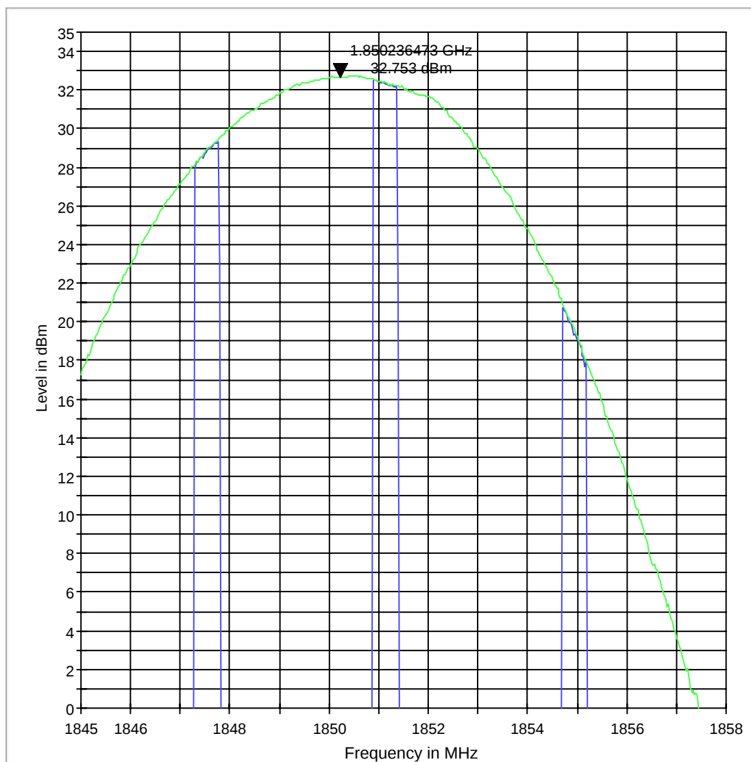
EIRP 1900 L
