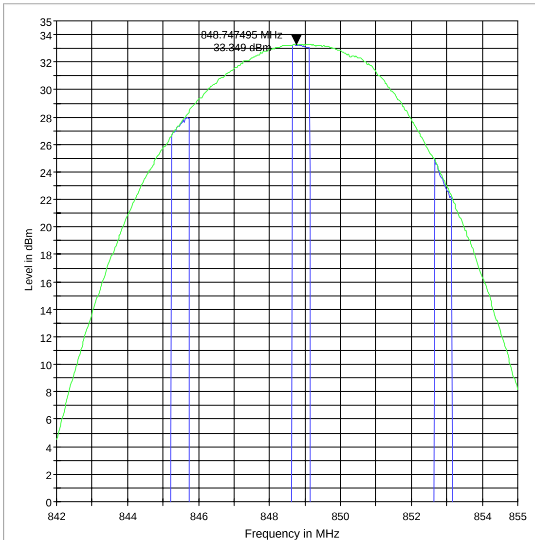
ERP 850 H
