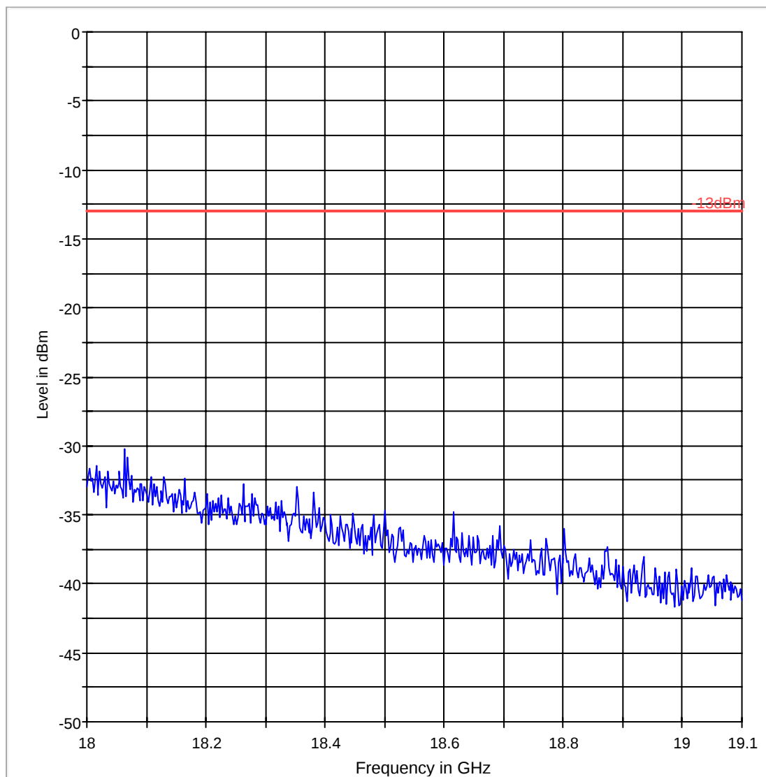
FCC 24 18-19.1GHz
