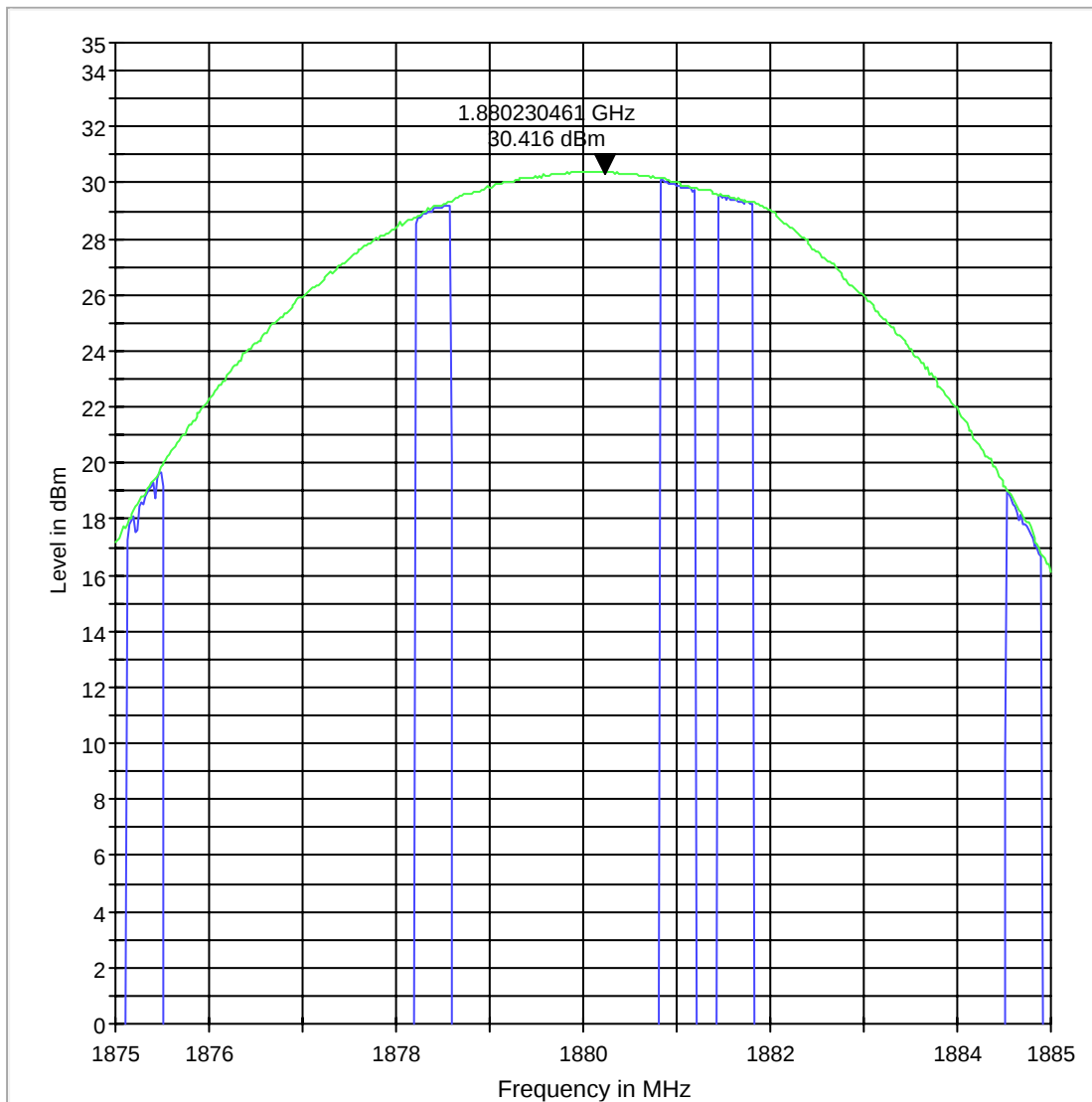
EIRP 1900 M
