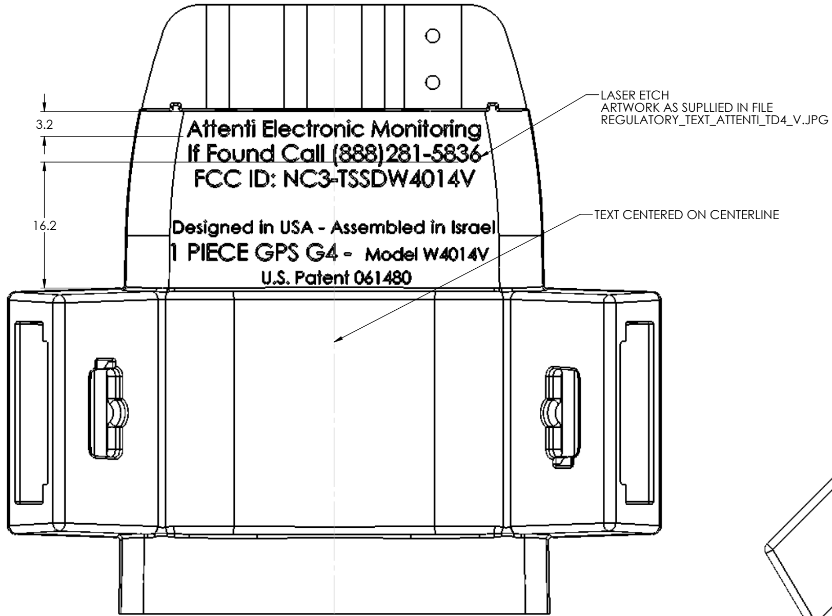
REAR/BACK VIEW
