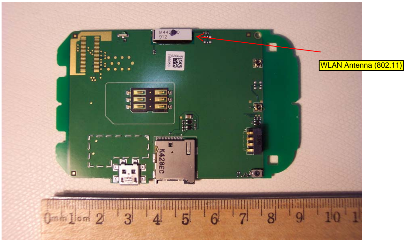
PCB Rear view
