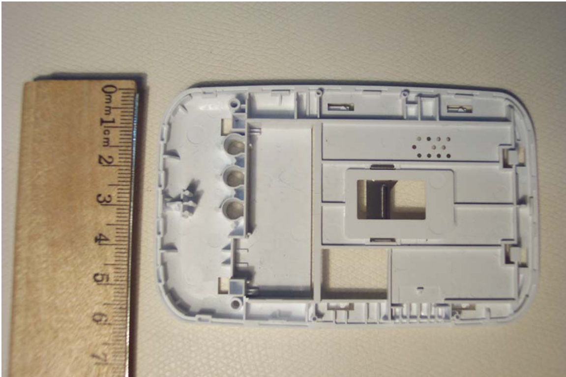
Front cover with antennas
