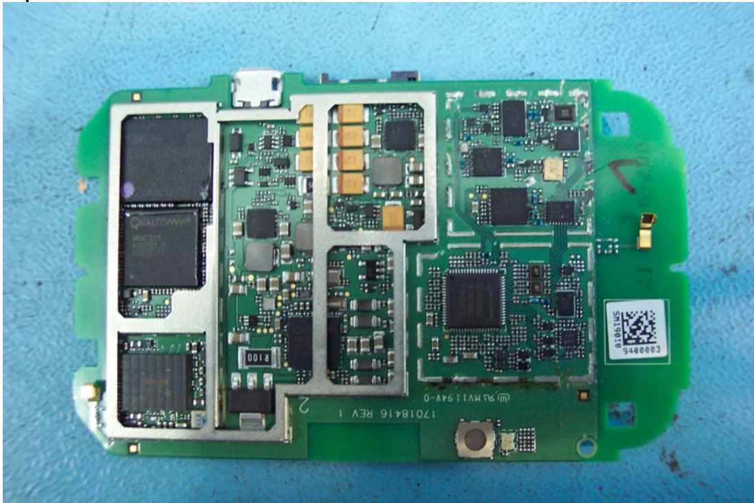
Top View of PCB without Shields
