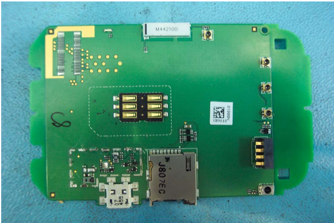
Bottom View PCB Shield Removed
