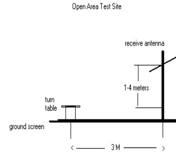
Figure 0-1. Diagram of 3-meter outdoor test range
