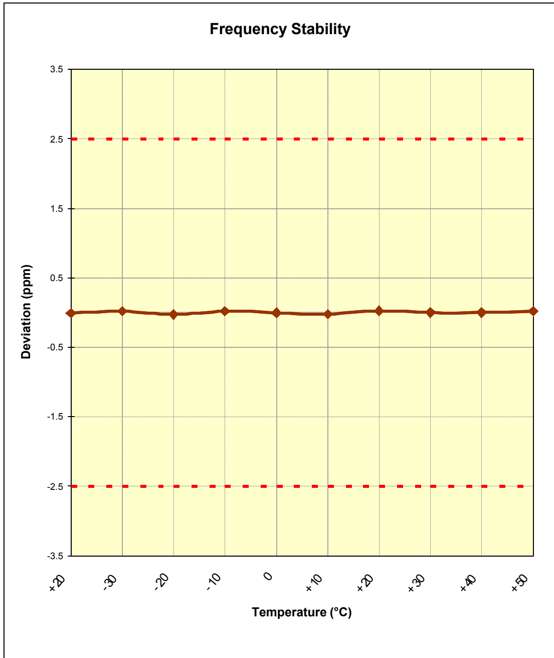
Plot 6-11. Frequency Stability Graph (Cellular GSM Mode – Ch. 190)
