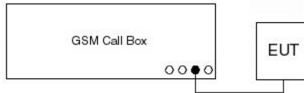
Figure 6-1 GSM Conducted Power Setup
