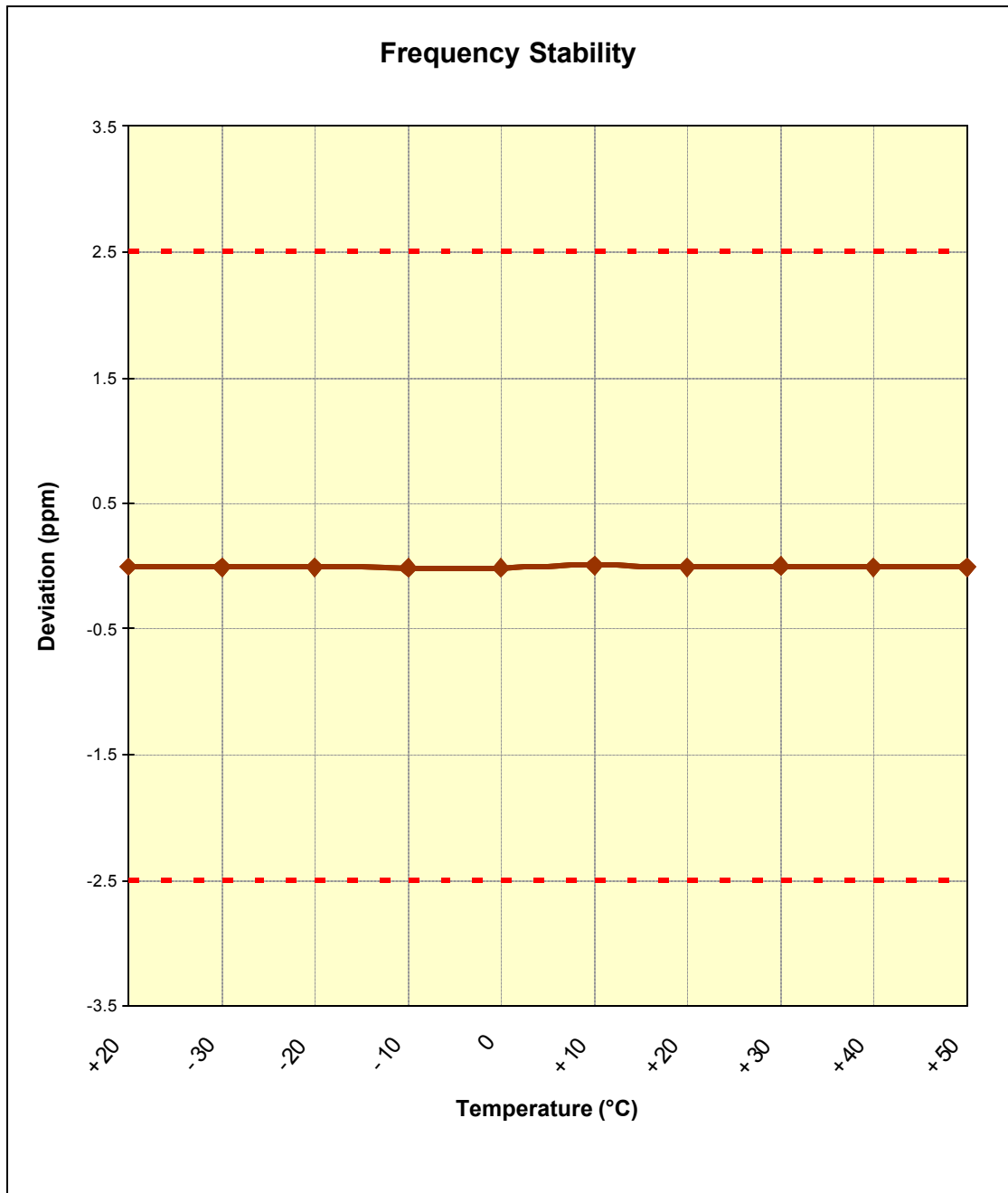
Plot 6-13. Frequency Stability Graph (PCS GSM Mode – Ch. 661)
