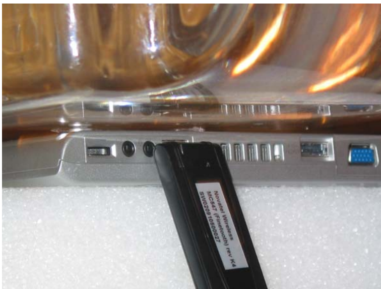
Bottom Test Configuration 5 mm Gap
