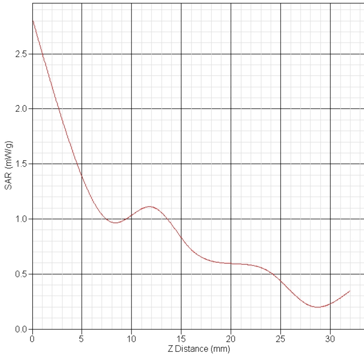
SAR-Z Axis at Hotspot x:15.06 y:-0.14
