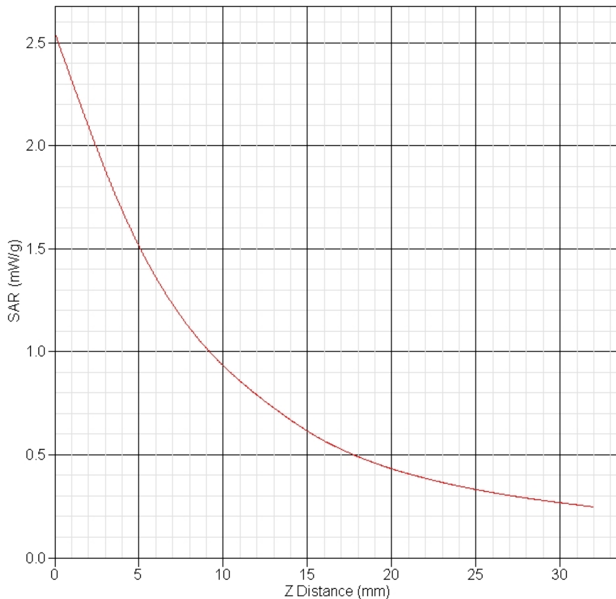
SAR-Z Axis at Hotspot x:15.02 y:7.89
