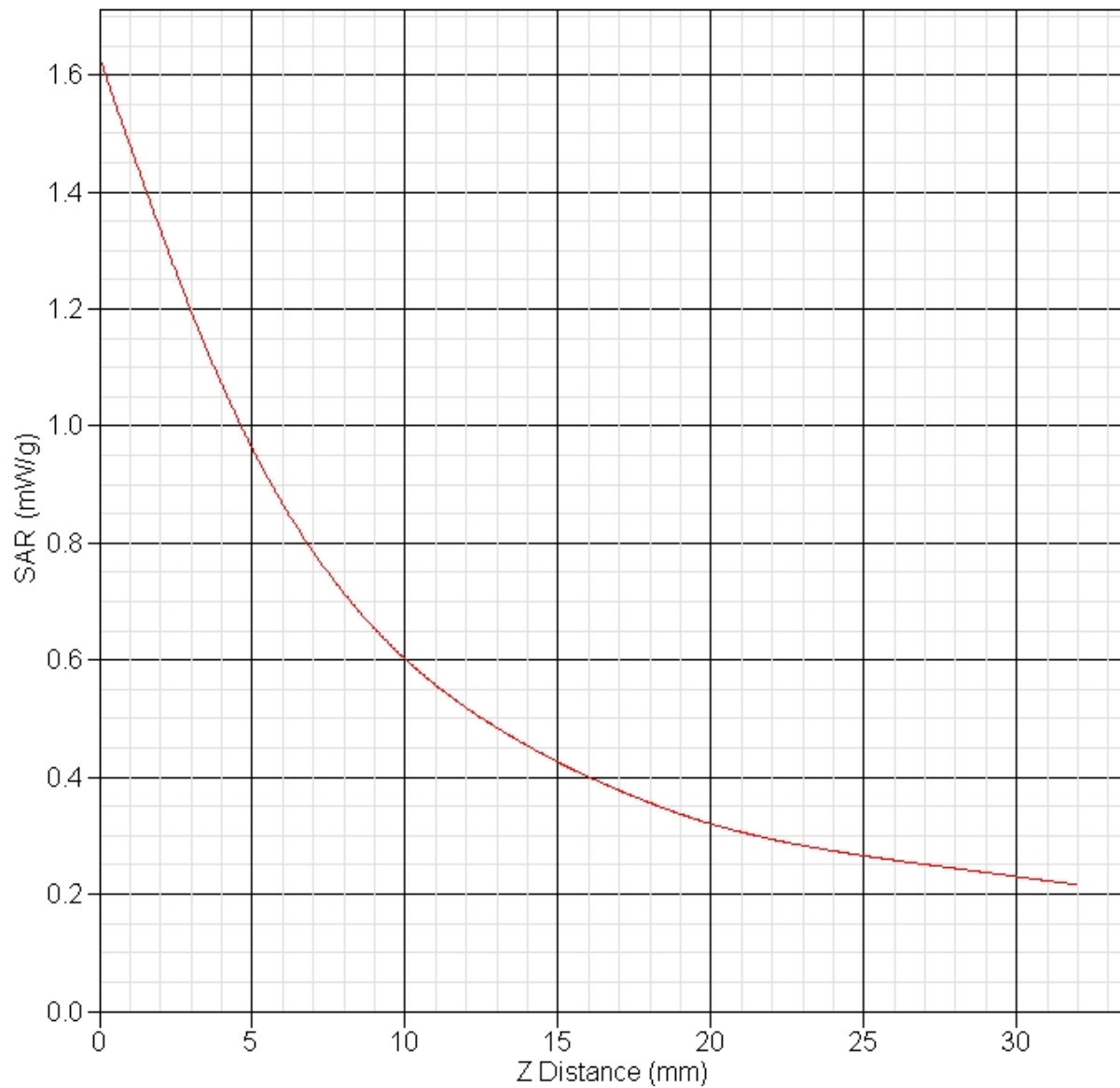
SAR-Z Axis at Hotspot x:23.01 y:7.86
