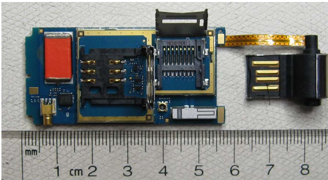
Rear view cover off (SIM and microSD connectors)
