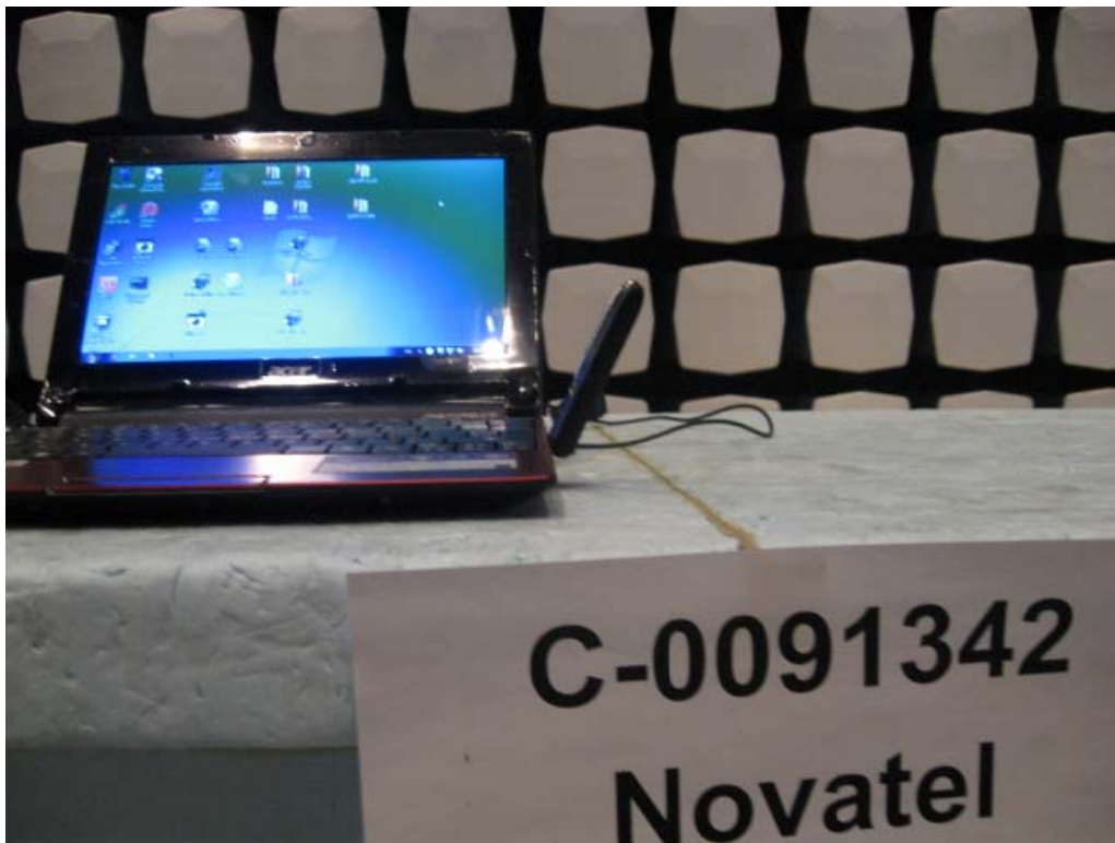
Radiated Emission
