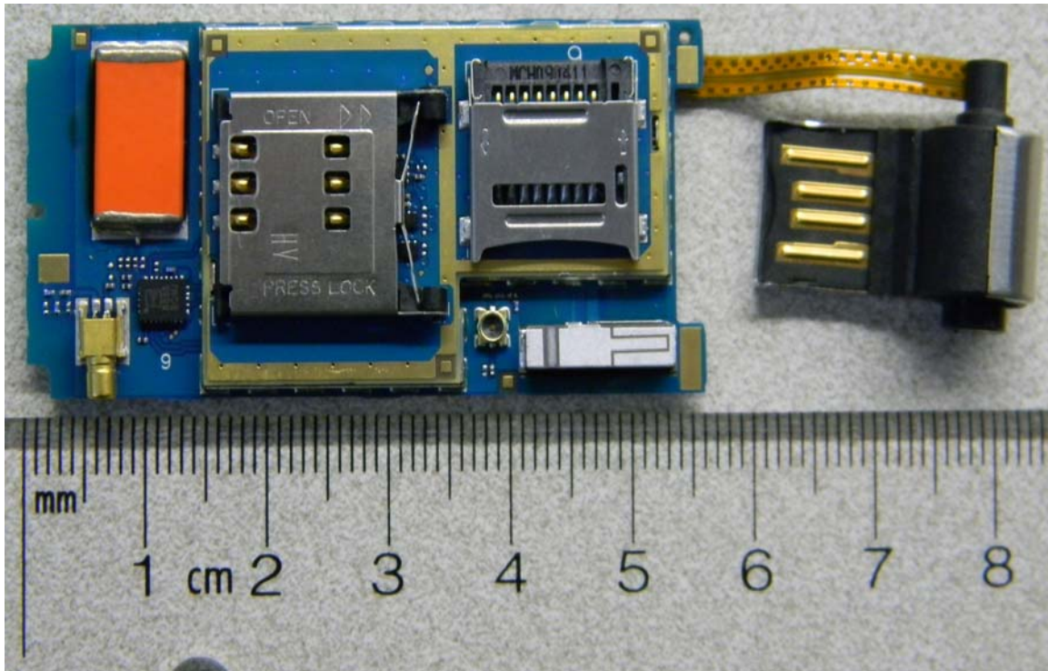
Rear view cover off (SIM and microSD connectors)
