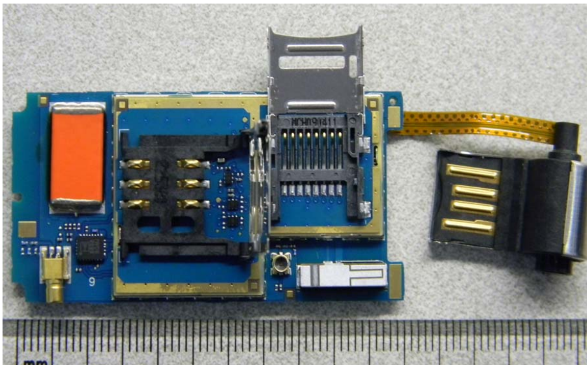
Rear view cover off (SIM and microSD connectors)
