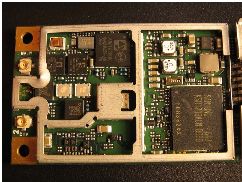
Top - Under Shield
