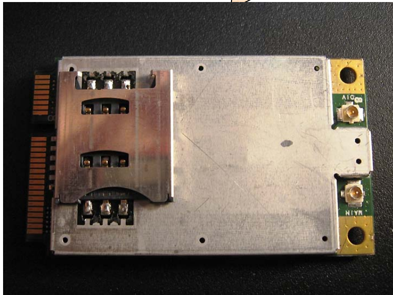
Top - Shield On
