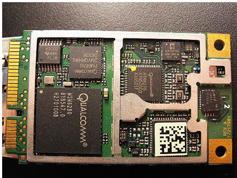
Bottom - Under Shield
